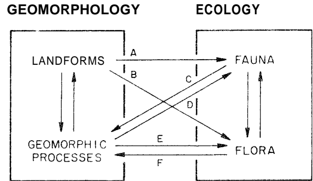
Figure 1. Relationships among landforms, geomorphic processes, fauna, and flora. A. Define habitat, range. Effects through flora. B. Define habitat. Determine disturbance potential by fire, wind. C. Affect soil movement by surface and mass erosion. Affect fluvial processes by damming, trampling. D. Sedimentation processes affect aquatic organisms. Effects through flora. E. Destroy vegetation. Disrupt growth by tipping, splitting, stoning. Create new sites for establishment and distinctive habitats. Transfer nutrients. F. Regulate soil and sediment transfer and storage.
