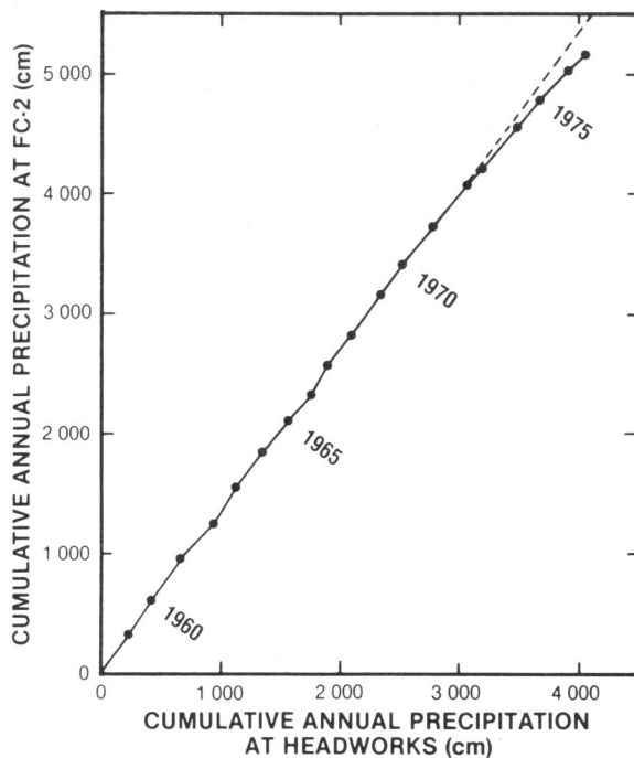
Figure 6.--Double-mass plot of cumulative annual precipitation at FC-2 and cumulative annual precipitation at Bull Run Headworks.
