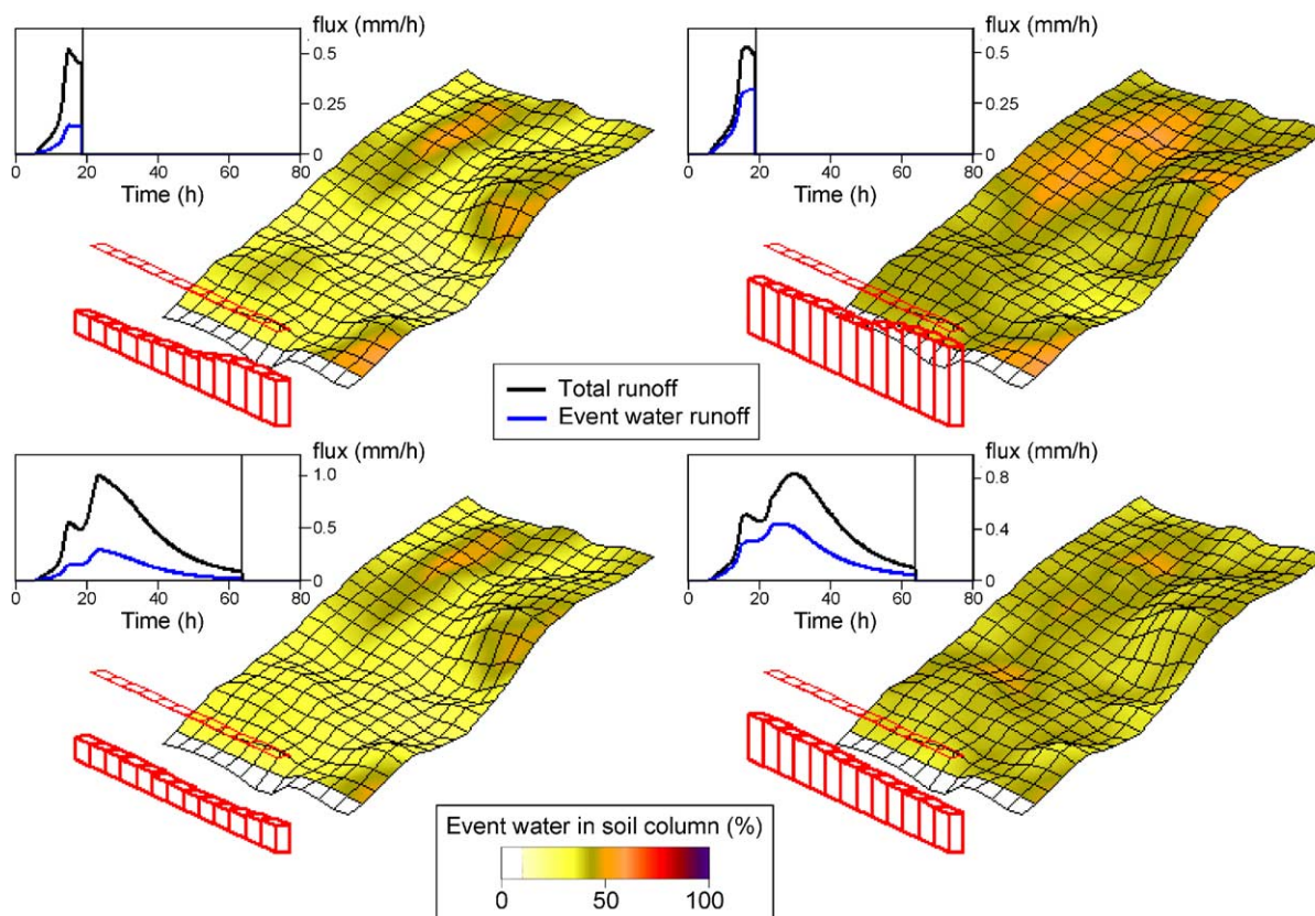
Fig. 6. Two snapshots of the virtual experiments for low and high drainable porosity, showing the dynamics of isotope tracing hydrograph separation described by the spatial variability of the event water percentage within the soil column (color coded values superimposed on the elevation mesh of bedrock topography), the spatial outflow variability of the proportion of event water compared to the 100% value (bar plot), and the outflow hydrograph of total runoff and event water runoff (flow–time plot, where the thin vertical line is indicating the actual step).
