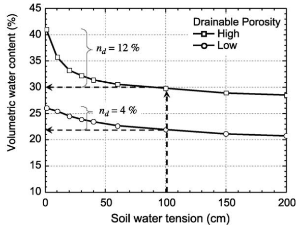
Fig. 2. Water retention characteristic for two soils based on data from the H.J. Andrews Experimental Forest, USA (Ranken, 1974), showing the determination of the drainable porosity based on the concept of field capacity and the water retention curve.
