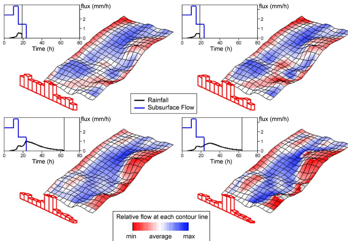
Fig. 3. Two snapshots of the virtual experiments for low and high drainable porosity, showing subsurface flow dynamics described by the spatial variability of relative flow along each contour line in the hillslope (color coded values superimposed on the elevation mesh of bedrock topography), the spatial variability of outflow (bar plot), the temporal variability of the rainfall and total subsurface runoff (flux–time plot, where the thin vertical line is indicating the actual step).
