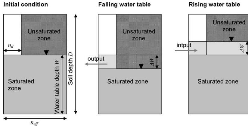
Fig. 1. Conceptualization of the mass exchange between the saturated and unsaturated zone, showing the parameter for the initial condition and the resulting changes for a falling water table (output > input) and a rising water table (output < input).
