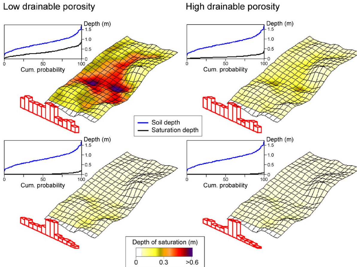
Fig. 4. Two snapshots of the virtual experiments for low and high drainable porosity, showing the dynamics of saturation depth described by the spatial variability of depth of saturation in the hillslope (color coded values superimposed on the elevation mesh of bedrock topography), the spatial variability of outflow (bar plot), and the cumulative soil depth and depth of saturation for the time step (soil depth–probability plot).
