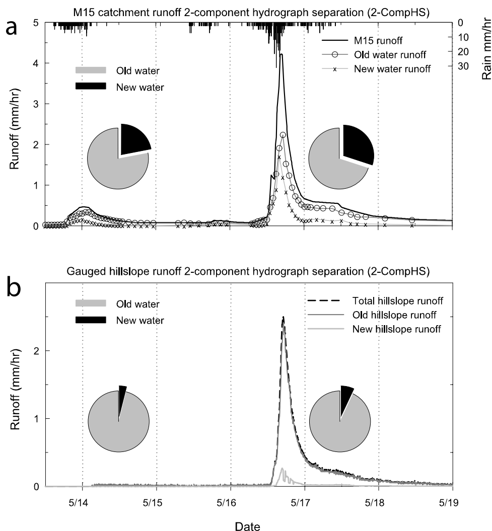
Figure 7. (a) Two-component temporal hydrograph separations of M15 catchment runoff into new and old water. Pie charts represent the relative proportions of new (solid) and old water (shaded) for events 1 and 2. (b) Two-component temporal hydrograph separations of gauged hillslope runoff into new and old water. Pie charts represent the relative proportions of new (solid) and old water (shaded) for events 1 and 2. Note the small proportion of new water in hillslope runoff in both events.
