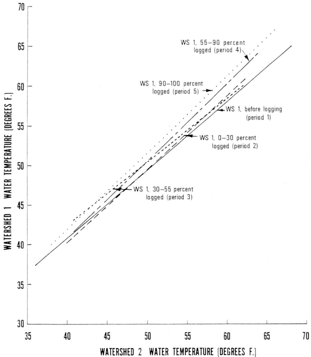
Figure 6.--Maximum weekly water temperature, watersheds 1 and 2.
