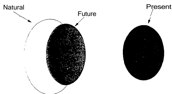
FIGURE 5.—Conceptual representation of the range of conditions experienced by aquatic ecosystems historically, currently, and under a new disturbance regime (modified from H. Regier, University of Toronto, personal communication).
