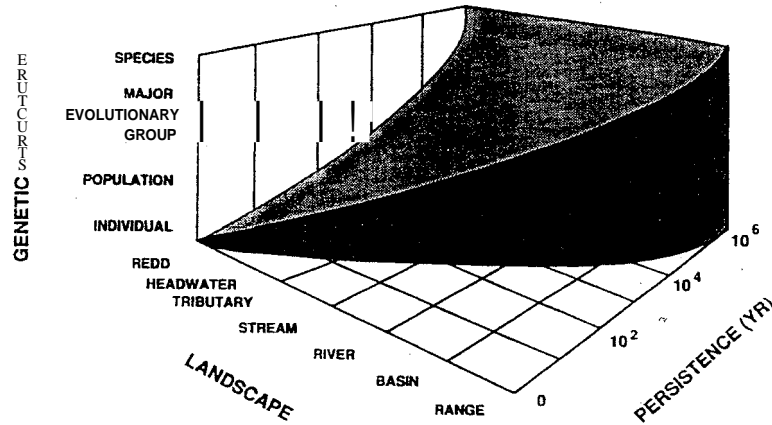
FIGURE 1.-A general hierarchical model of biological levels of organization for anadromous salmonids and the spatial and temporal scales that influence them (from Currens et al., in press).
