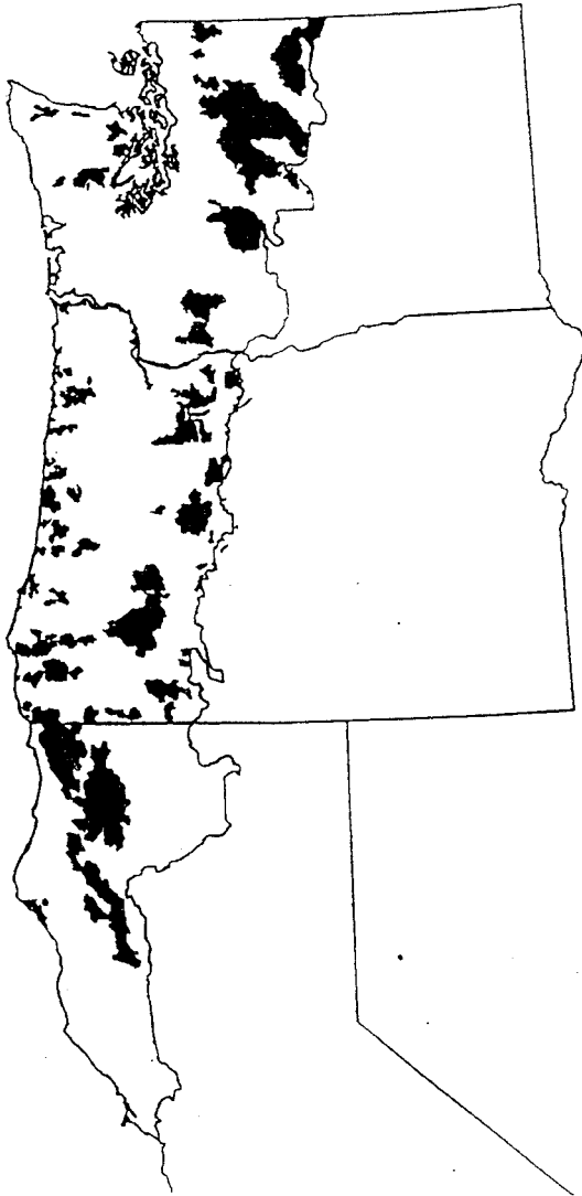
FIGURE 4.—Distribution of tier 1 key watersheds identified by Thomas et al. (1993).
