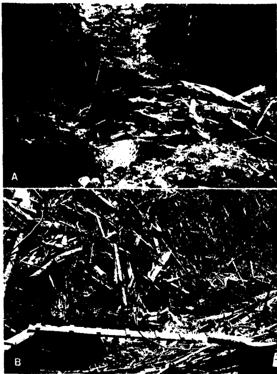
FIG. 1. (A) A log debris dam in Mack Creek at H. J. Andrews Experimental Forest, and (B) logging debris on the forest floor and in the small stream draining Watershed 10.
