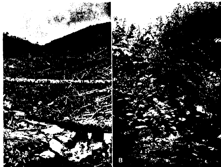
FIG. 2. (A) Big Hurricane Branch in 1977, shortly after the watershed was logged, and (B) the same site in 1983, 6 yr after logging. Big Hurricane Branch drains Watershed 7 at Coweeta Hydrologic Laboratory.
