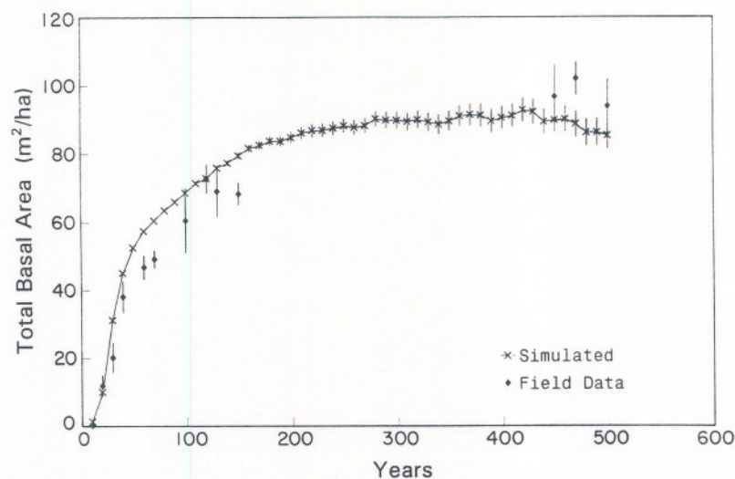
FIG. 4. Trends in total basal area under natural succession at 1000 m elevation, western slope of the Oregon Cascades mountains as described by field data and as simulated with the gap model ZELIG.PNW (see Step 4 . . . : Example: Models). Simulated data are based on 30 model plots. Sample sizes of field data varied from 5 to 42 reference stands. Data shown are means \pm 1 SE.
