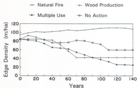
FIG. 7. Density of edges among seven seral stages in the planning area under the four management scenarios.
