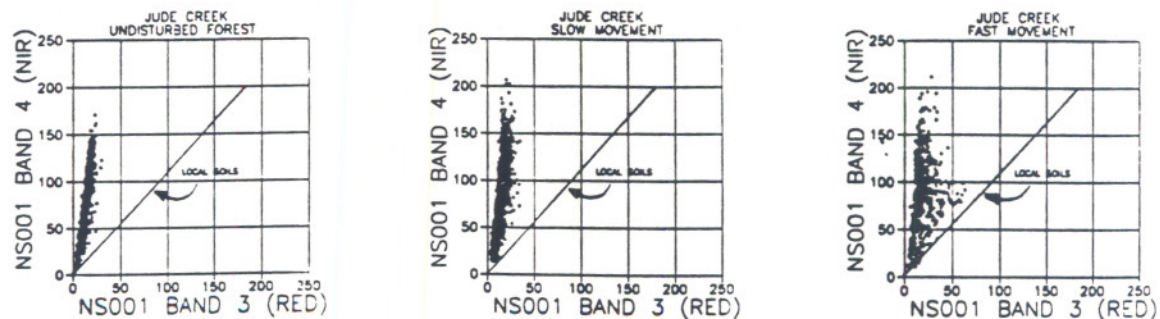
FIG. 11. Jude Creek earthflow reflectance values.
