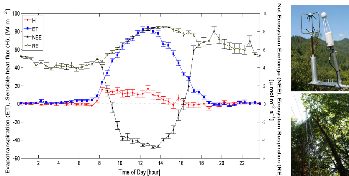
Figure 4: a) Mean diurnal courses of net ecosystem exchange of \text{CO}_2 (NEE), ecosystem respiration (RE), evapotranspiration (ET), and sensible heat (H) and standard error (vertical bars) for the dry summer period July 25–October 2, 2012 measured at the WS1 eddy covariance tower computed using the modified mass balance approach that accounts for advective losses of carbon dioxide in the carbon mass balance (Thomas et al., 2008; 2013; 2014, submitted) due to limited vertical mixing and the persistent cold-air drainage; b) The eddy covariance system at the top of the WS1 tower above the main forest canopy; c) View of the 38.5m tall ecosystem flux tower that features 8 levels of concentration measurements of ^{13}\text{CO}_2 , ^{12}\text{CO}_2 , \text{CH}_4 , \text{H}_2\text{O} , and air temperature in a vertical profile, and 2 eddy covariance systems (at 38.5m and 4m).
