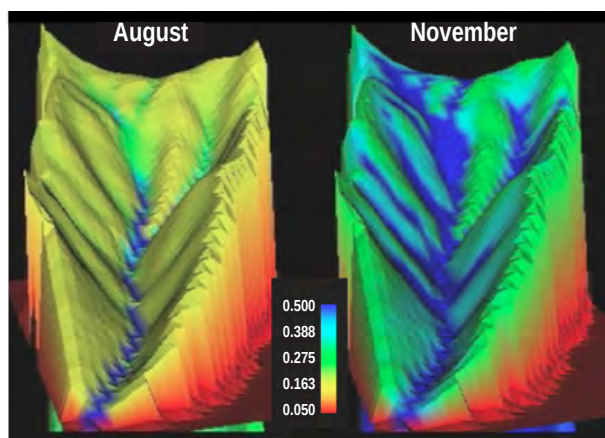
Figure 7. Soil moisture content by volume fraction simulated by VELMA (Abdelnour et al. 2012, 2013) for the steep forested slopes of Watershed 1 in the Andrews Forest. This visualization of model output shows the contraction of the stream network and associated area of moist soils in late summer (mid-August) and the expansion of the stream network and moist areas during the wet season (November to April). An extensive soil moisture monitoring network in LTER7 will provide data to test and refine models of spatiotemporal patterns of moisture and to relate small-scale moisture variability to plant productivity.
