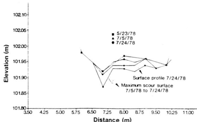
Figure 8.--Cross section 1, lower zone 3, drainage basin 1200. Lower profile for 7.24.78 is the surface of greatest scour during the survey interval. Upper profile for 7.24.78 is existing surface at time of survey.
