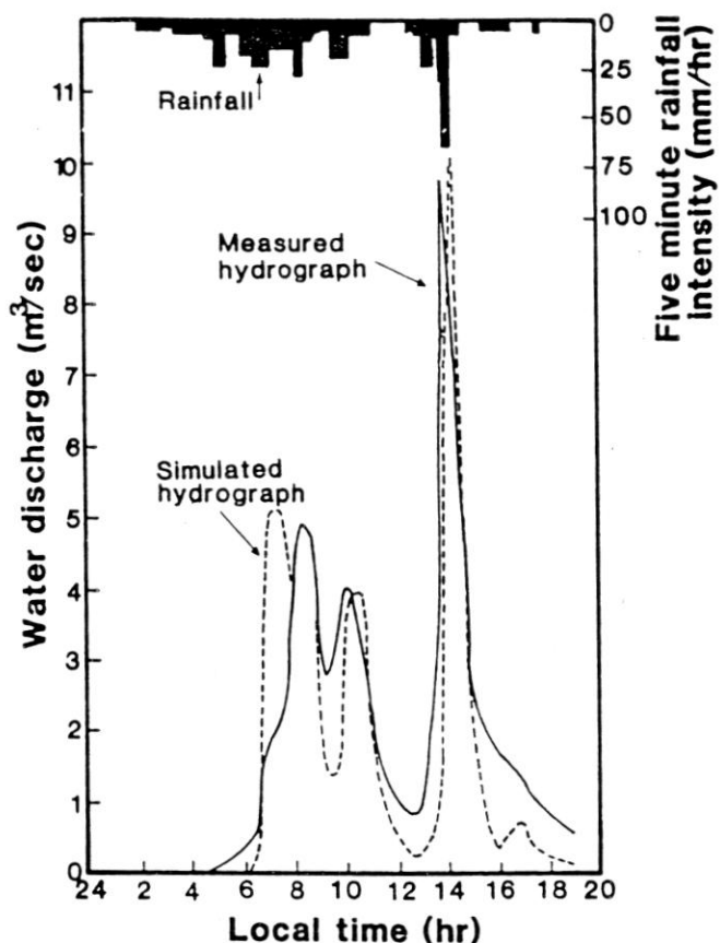
Figure 3.--Water hydrograph from Watershed 17 for the September 5, 1970 storm (after Simons et al. 1975).
