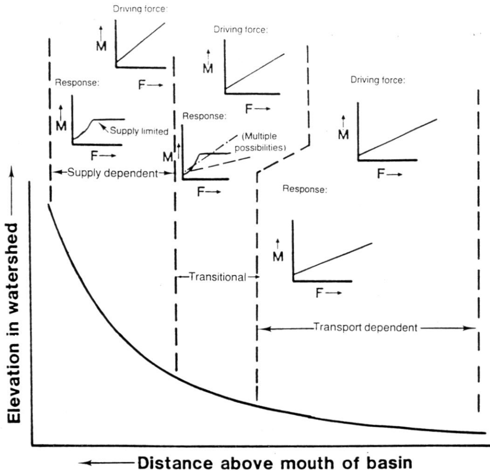
Figure 3.--Summary diagram showing possible relationships of magnitude ( m ) and frequency ( f ) of driving force and geomorphic response at different sites within a fluvial system. Sites are depicted on a schematic version of a longitudinal stream profile.
