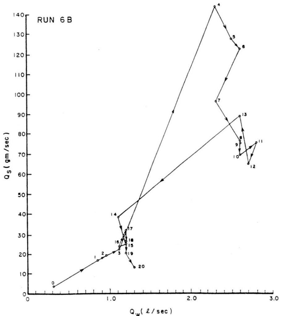
Figure 5.--Hysteresis loops of total sediment and water discharge for Run 6.
