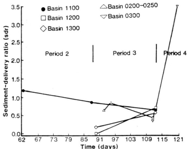
Figure 2.--Change of sediment-delivery ratios with time for five tributary basins.
