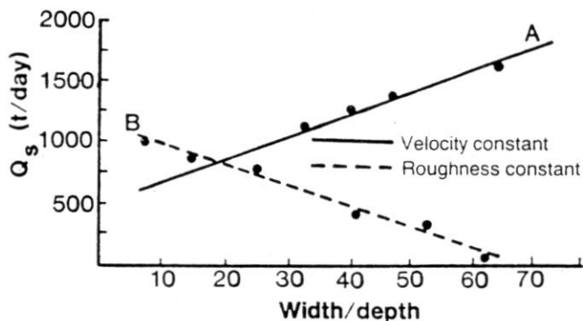
Figure 5.--Rates of sediment transport at various width-to-depth ratios.
