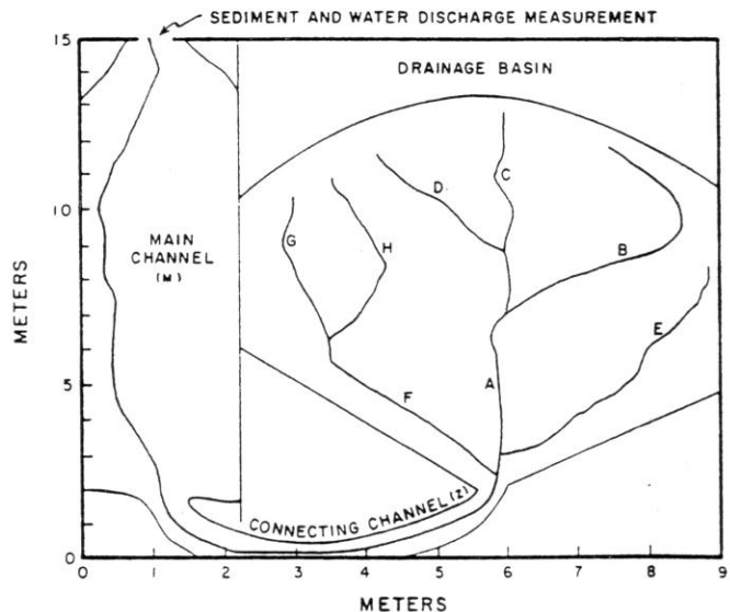
Figure 1.--Plan view of R.E.F. showing drainage basin, connecting channel (Z), main channel (M), and measuring point.
