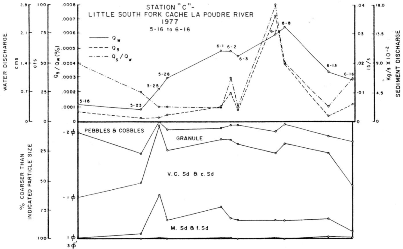
Figure 9.--Water and sediment discharge and sedimentology for 1977 runoff season, South Fork, Cache la Poudre River, Colorado.
