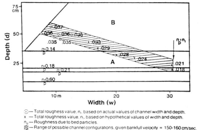
Figure 6.--Velocity and roughness constraints on the Big Beef Creek channel configuration at bankfull discharge (relationships determined from equations 3, 4, and 6).
