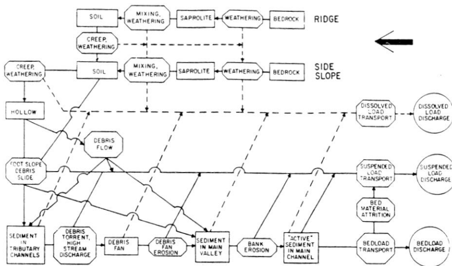
Figure 2.--Sediment-budget model for the Rock Creek basin, central coastal Oregon: rectangles, storage sites; octagonals, transfer processes; circles, outputs; solid lines, transfer of sediment; and dotted lines, migration of solutes (from Dietrich and Dunne 1978).
