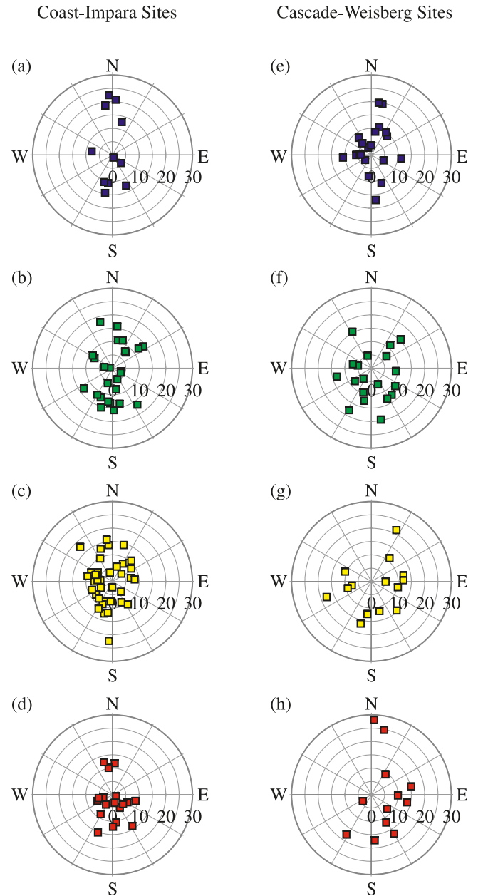
Fig. 6. Slopes and aspects for sites in the (a–d) Coast-Impara (site numbers 11–103) and (e–h) Cascade-Weisberg (site numbers 125–190) areas. Symbol color indicates age structure group. Slope (degrees) increases with distance from the center of each polar plot.
