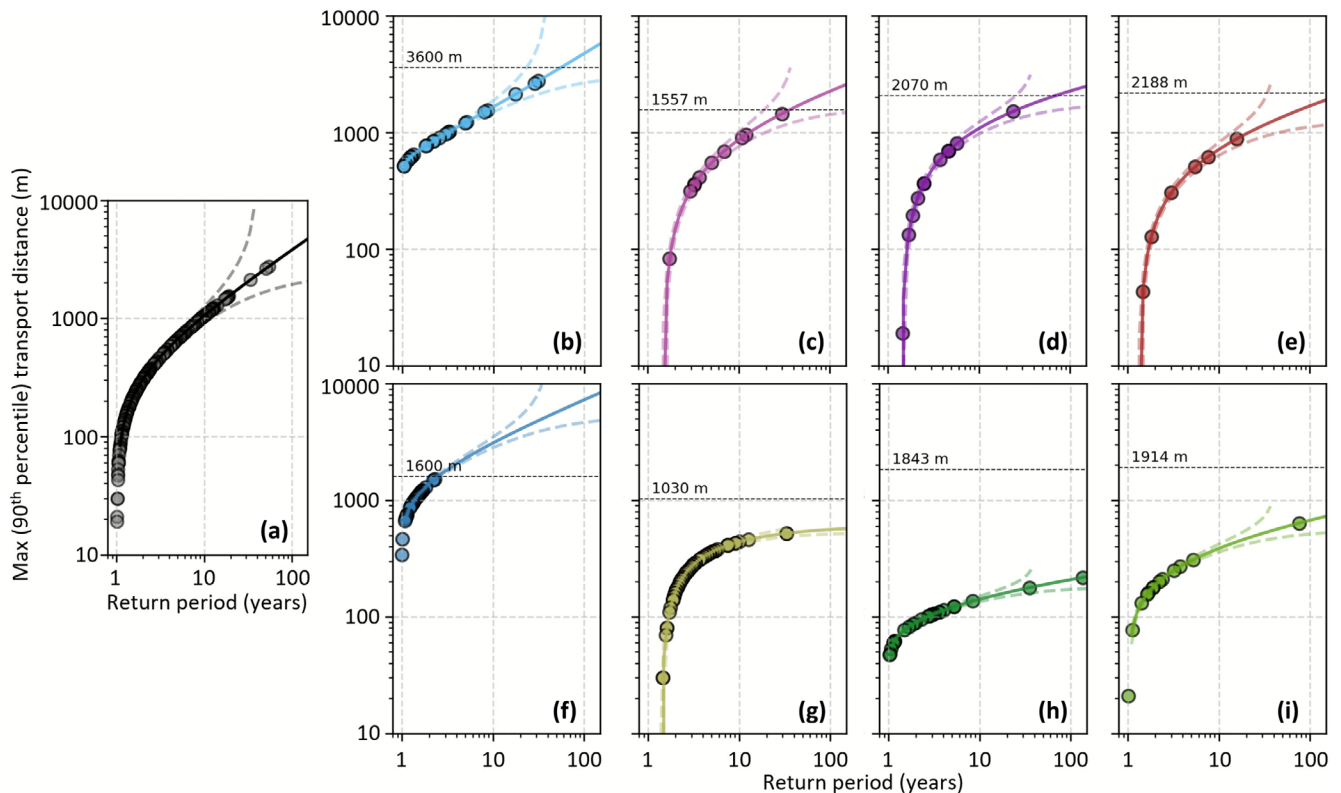
FIGURE 12 Return periods, in years, for maximum transport distances (based on the 90th percentile of observations per year), in meters, of mobilized wood for a) all of the rivers combined and eight rivers, b) Spöl, c) Vuelta de Zorra, d) Tres Arroyos, e) El Toro, f) Avançon de Nant h) Mack Creek, h) north fork, Caspar Creek, i) south fork, Caspar Creek, based on general extreme value distribution. Highland water, Poplar Creek and Pichún are included in the combined ( n < 6 ). The dashed black line, in each panel, represents the length of the river survey. See Table 4 for exact values per return period.
