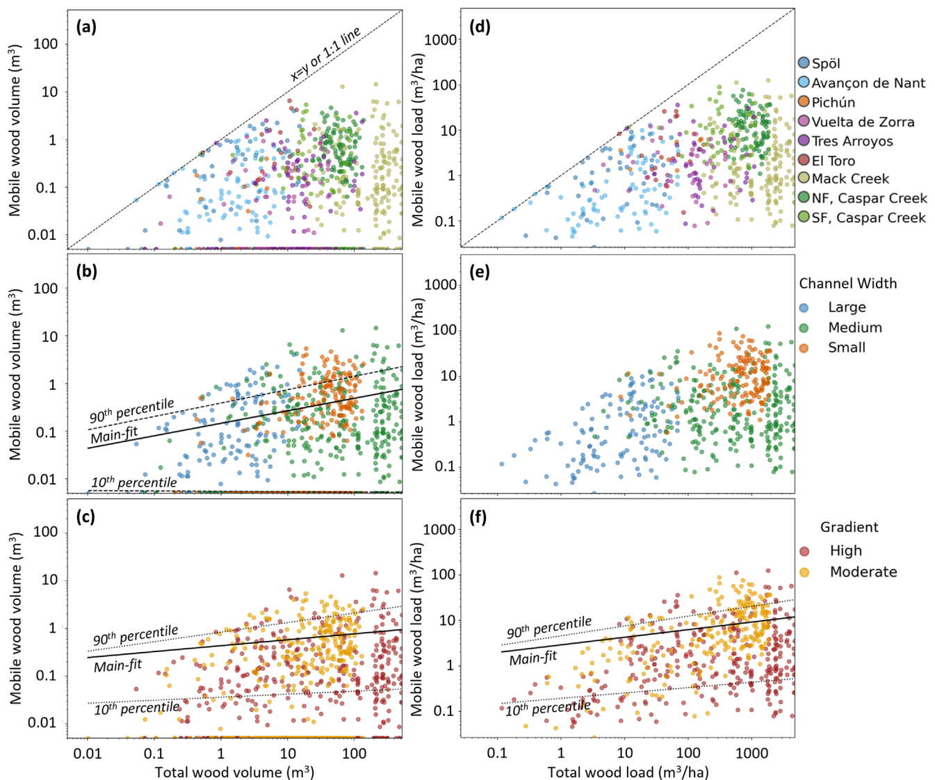
FIGURE 6 Scatter plots of mobile wood volume ( \text{m}^3 ) and total wood volume ( \text{m}^3 ) for a) individual rivers, b) channel width classifications and c) channel gradient classifications. Panels d, e and f are those classifications, respectively, but by wood load ( \text{m}^3/\text{ha} ). Each point represents a reach per event per dataset. For wood volume panels (a-c), reaches in which wood was present but no pieces were observed to move were assigned an arbitrary low value of 0.005 \text{ m}^3 for plotting on the log scale ( n = 588 ; n_{\text{total}} = 1,076 ). These zero-movement cases appear along the lower edge of each plot. The dashed line in panel a represents mobile wood volume equaling total wood volume. In panel b, the 90th- and 10th-percentile power-law fits are shown as dashed lines, and the main fit is shown as a solid line, and they include the zero ( 0.005 \text{ m}^3 ) values in the fit. The power-law coefficients (a, b) for the main, 10th-percentile, and 90th-percentile fits were (0.15, 0.26; R^2 = 0.03 ), (0.005, -0.008 ) and (0.39, 0.28), respectively. Panel c excludes the zero values during fitting, and power-law coefficients for the main, 10th-percentile, and 90th-percentile fits were (0.43, 0.12; R^2 = 0.02 ), (0.04, 0.06) and (0.83, 0.20). Panel f includes the main, 10th-percentile, and 90th-percentile power-law fits based on wood load, which were (2.88, 0.17; R^2 = 0.04 ), (0.19, 0.12) and (4.56, 0.22). The relationship for low gradient rivers could not be computed due to data availability.
