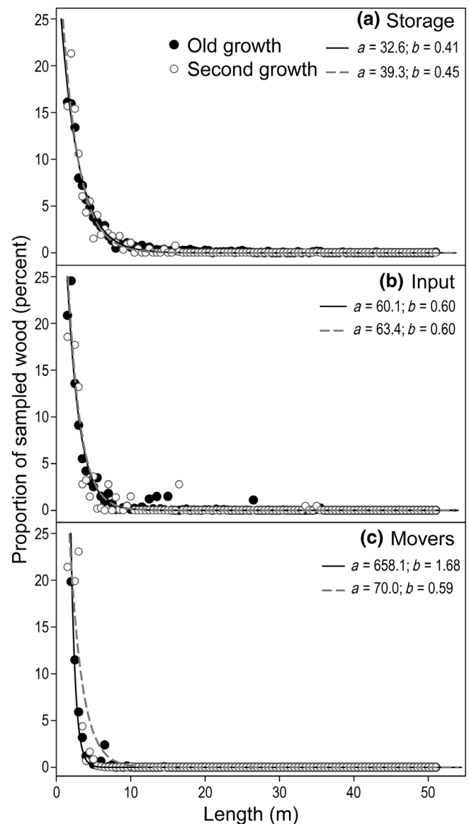
FIGURE 9 Percent of size classes of total large wood storage, input, and movers per 100 m in the old-growth and second-growth reaches of Mack Creek from 1985 to 2008. Curves are based on an exponential decay equation ( Y = a \cdot \exp(-b \cdot X) ).
