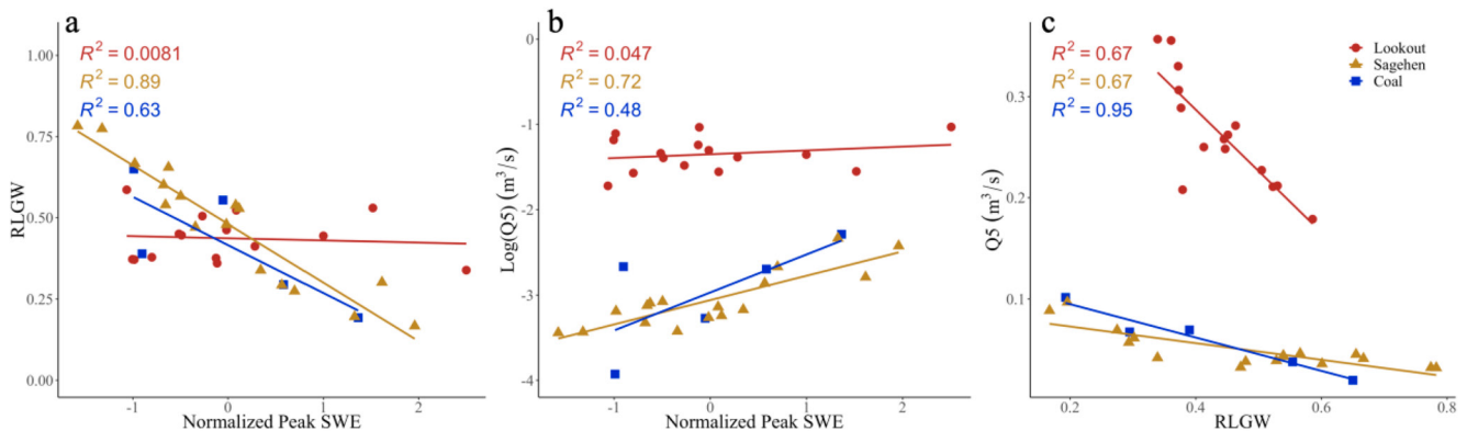
Figure 4. Linear relationships between annual (a) recession limb groundwater (RLGW) and z -score normalized peak snow water equivalent (SWE), (b) \log Q_5 and z -score normalized peak SWE, and (c) Q_5 and RLGW for Lookout Creek (red circle), Sagehen Creek (yellow triangle), and Coal Creek (blue square).
