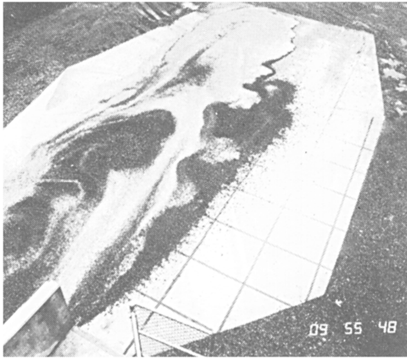
Fig. 3: Deposit formed by the debris flow shown in figure 2. A one-meter grid on the runout surface provides scale
