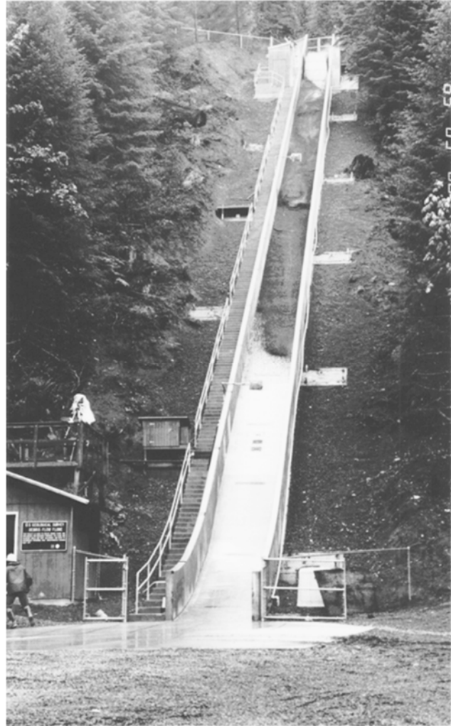
Fig.2: An experimental debris flow descends the flume
