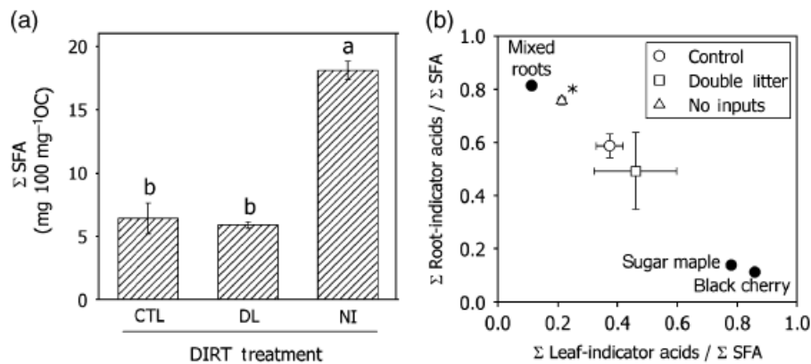
Fig. 2 Bulk soil SFA yield (a) and the relative proportion of root-indicator acids vs. leaf-indicator acids for bulk soil and plant litter (b) for the Bousson DIRT plots. Values are means \pm 1 standard error; letters indicate significant differences among treatment mean \Sigma SFA values; *Significant differences between both variables for that treatment compared with the others; see Table 3 and text for P -values.
