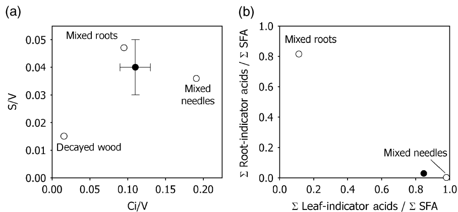
Fig. 4 Comparing ratios of lignin-derived phenol classes (a) and the relative proportion of root-indicator acids vs. leaf-indicator acids for bulk soil (solid symbols) and plant litter (open symbols) (b) at the H.J. Andrews DIRT plots. No significant differences existed among the DIRT treatments, values are site means \pm 1 standard error.
