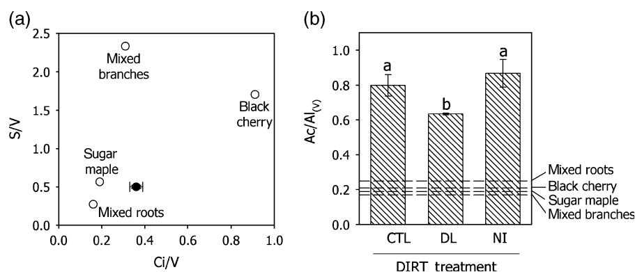
Fig. 1 Comparing ratios of lignin-derived phenol classes for bulk soil (solid symbol) and plant litter (open symbols) (a) and the acid-to-aldehyde ratio of V-Lignin for bulk soil (bars) and plant litter (dotted lines) (b) at the Bousson DIRT plots. Values are means \pm 1 standard error; letters indicate significant differences among means for the treatments; if no differences existed, the site mean is shown; see Table 3 for P -values.
