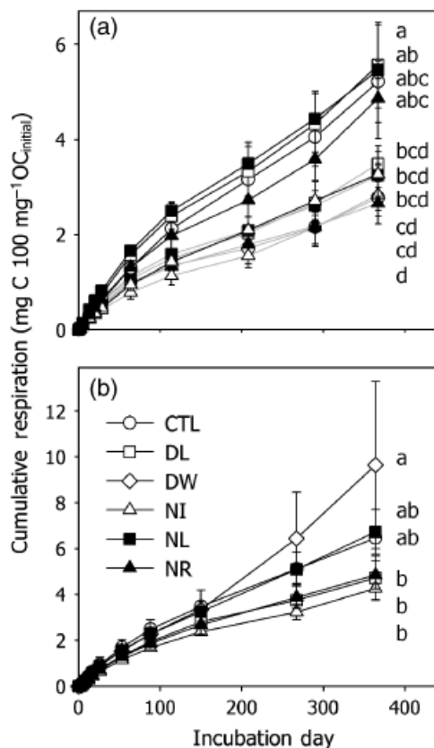
Fig. 3 Cumulative respiration during a 1-year incubation of soil light fraction (black lines) and heavy fraction (grey lines) from the Bousson DIRT plots (a) and bulk soil from the H.J. Andrews DIRT plots (b). Values are means \pm 1 standard error; letters indicate significant differences among means, see text for P -values. Note that (a) and (b) are on different scales.
