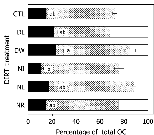
Fig. 5 Partitioning of bulk soil OC among the light fraction (black bars), heavy fraction (hatched bars), and SPT-soluble fraction (white bar) at the H.J. Andrews DIRT plots. Values are means \pm 1 standard error; the soluble fraction was calculated by difference; letters indicate significant differences among means for the treatments, P = 0.097 .
