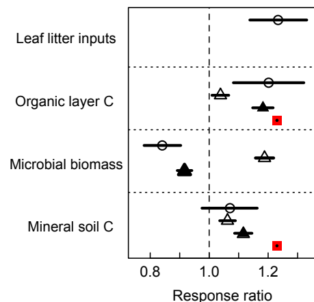
Figure 3. Observed and modeled C response ratio (treatment/control) to experimental N enrichment. Open circles show observed mean and 95 % confidence interval of leaf litter inputs, organic layer C, microbial biomass, and mineral soil C (Liu and Greaver, 2010). Modeled results show the steady-state changes in pools following increases in leaf litter inputs projected by MIMICS (open triangles), MIMICS (with increasing MGE in response to N enrichment; filled triangles) and DAYCENT (filled squares; see also Supplementary Fig. 1).
