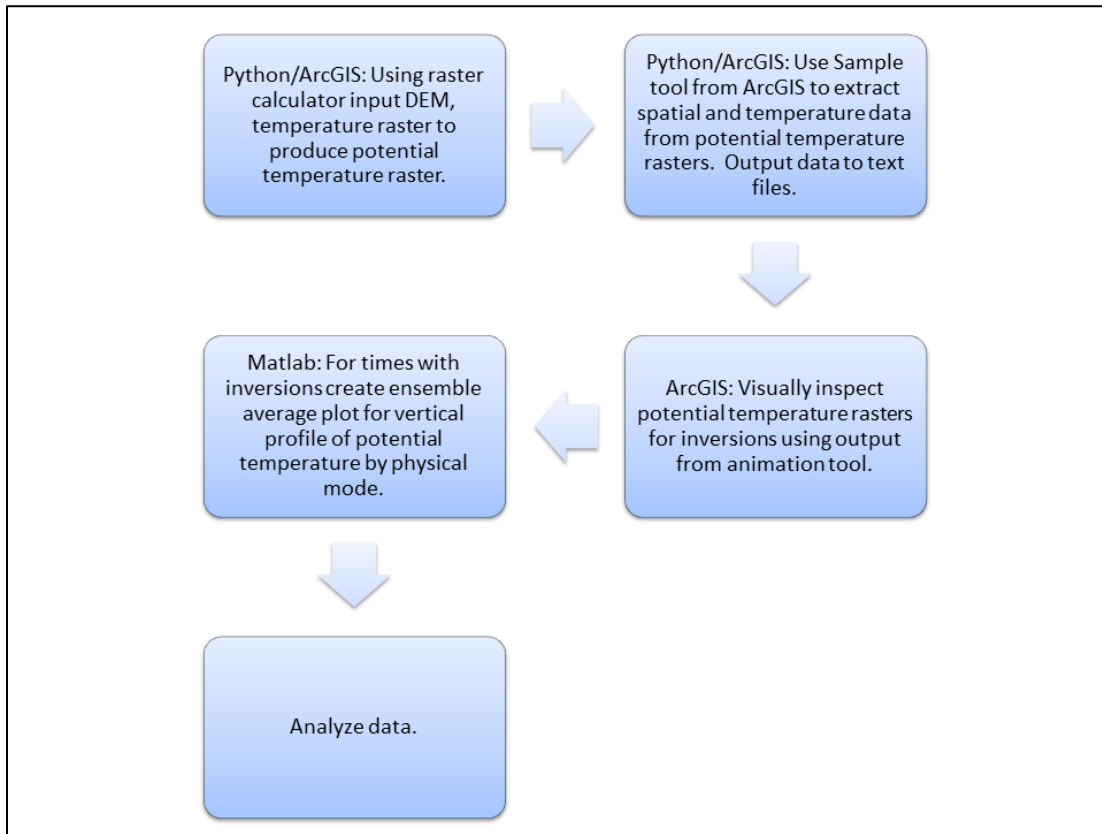
Figure 14: The geoprocessing workflow was developed to output plots of potential temperatures at 10 meter vertical elevation intervals. First spatially referenced temperature data were used to compute spatially referenced potential temperature data using Python/ArcGIS. Then an existing tool in ArcGIS was used to extract spatial information and potential temperature data from the raster. This information was written to a text file. Also, to quickly inspect the potential temperature rasters, the time series of data was animated for easy visual review. After noting times of interest, Matlab was used to input the text file based data, bin and average the potential temperatures, create confidence intervals, and output plots based on the flow regime in the watershed.
