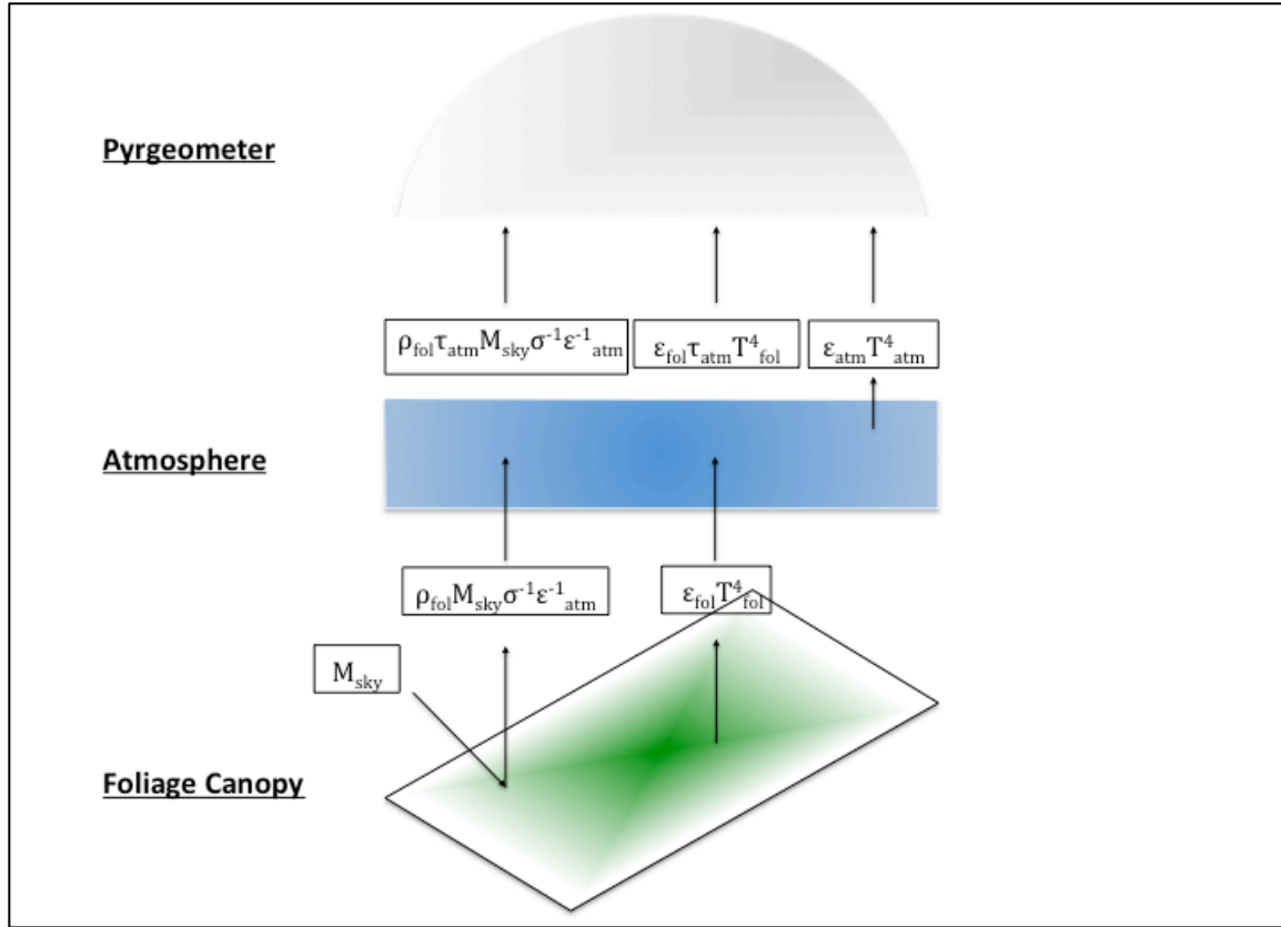
Figure 11: A conceptual representation depicting the foliage canopy, atmosphere, and thermal reflections sensed by the pyrgeometer.
