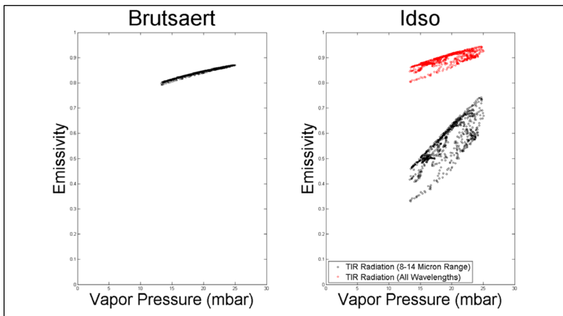
Figure 15: Atmospheric TIR emissivities as derived from Brutsaert's and Idso's formulations. The emissivity derived from Brutsaert's work accounts for a broad range of TIR wavelengths. The formulations developed by Idso are (in black) for the 8- \mu m to 14- \mu m range of the TIR spectrum and (in red) the entire TIR spectrum.
