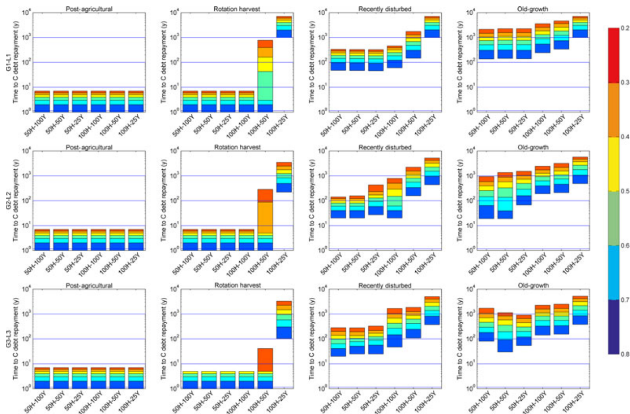
Fig. 2 Comparisons of the time required for a repayment of the C Debt Repayment among three of our nine ecosystem types, each with six biomass harvesting regimes and four land-use histories. Note that times are represented on a log scale. Different harvesting regimes are indicated on the x-axis, with 50% and 100% harvesting intensity represented as 50H and 100H, respectively. Harvest frequencies of 25, 50, and 100 years are represented as 25Y, 50Y, and 100Y.
