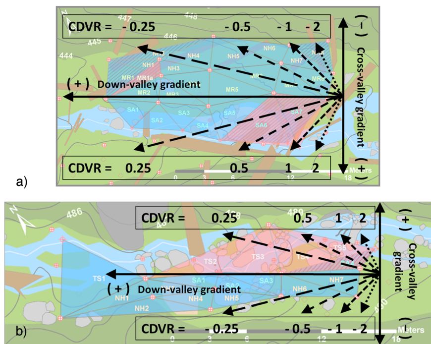
Figure 4. Illustration of the physical meaning of different hypothetical values of the cross- to down-valley ratio (CDVR), for (a) WS01 and (b) WS03. Note that the cross-valley sign convention for WS03 is opposite that of WS01, so that in both cases, a positive CDVR indicates a gradient directed towards the stream channel.
