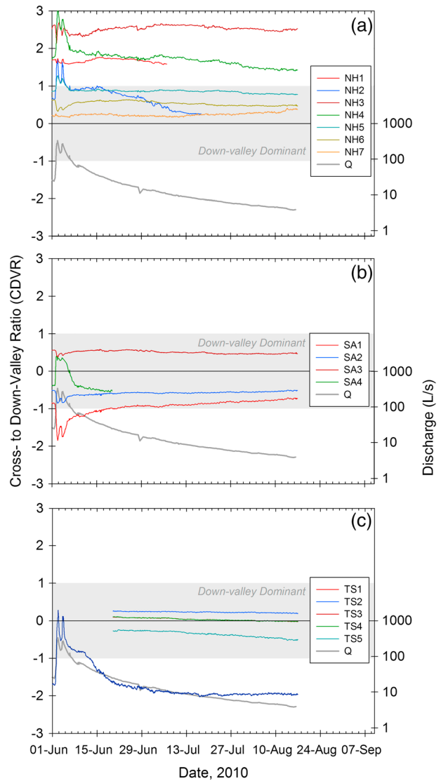
Figure 6. WS03 cross- to down-valley hydraulic gradient ratio (CDVR) for the entire field season, for (a) the near-hillslope zone, (b) the stream-adjacent zone, and (c) the through-stream zone. The grey band indicates the region of down-valley dominance (i.e., where |\text{CDVR}| < 1 ). Tick marks are displayed at 00:00 on the day labeled.
