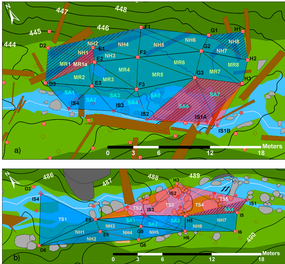
Figure 3. Riparian areas divided into near-hillslope (NH), middle-riparian (MR), stream-adjacent (SA), and through-stream (TS) zones for (a) WS01, and (b) WS03. Triangular elements with hatching denote gradient records that ended before the end of the season, and red-shaded elements are those that began part-way through the season, due to drying of wells.
