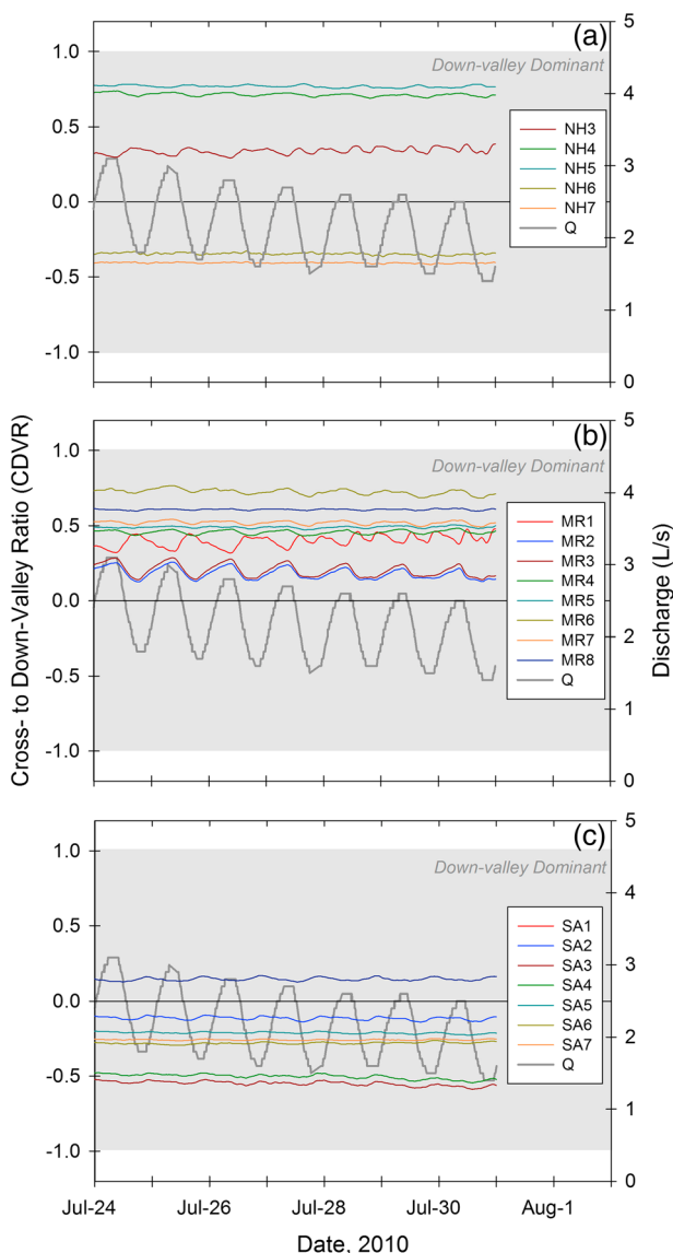
Figure 11. WS01 cross- to down-valley hydraulic gradient ratio (CDVR) for the period from 24 to 31 July for (a) the near hillslope zone, (b) the middle riparian zone, and (c) the stream adjacent zone. Tick marks are displayed at 00:00 on the day labeled.
