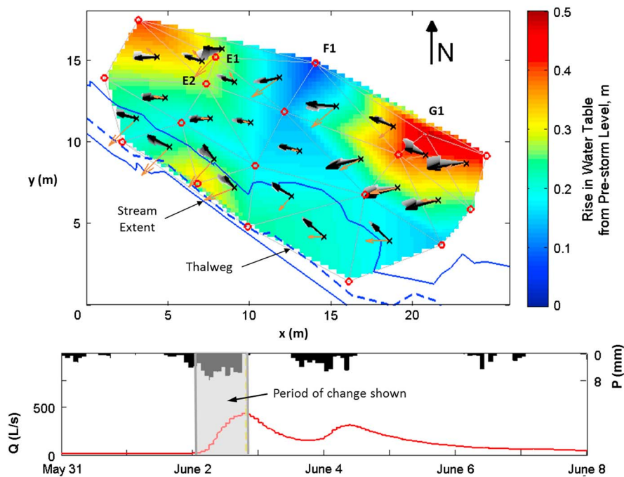
Figure 8. Time-lapsed image of the riparian hydraulic gradient storm response in WS01. Red circles indicate locations of water level measurement. Hydraulic gradient arrows (originating at x 's) are plotted such that the arrow color transitions from light grey to black as time progresses over the storm response period. Brown arrows show the surface topographic gradients at the centroid of each element. The colored background indicates the rise in water level from the pre-storm level, to show how water levels rose to produce the observed gradient changes. Flow is from bottom right to top left. Tick marks are displayed at 00:00 on the day labeled. Hydrograph ( Q ) in red and hyetograph ( P ) in black are presented in the bottom panel.
