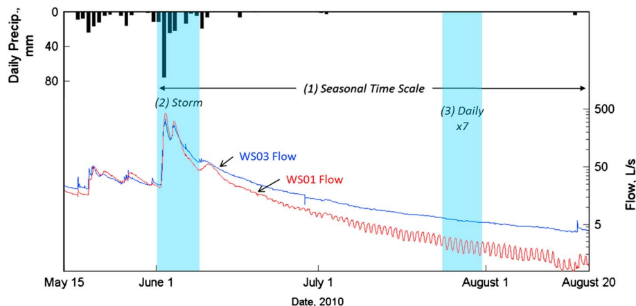
Figure 2. Hyetograph and hydrograph showing hydrologic conditions for the seasonal baseflow recession, and the time scales considered in our assessment. The daily timescale is shown for a typical 7 day period during baseflow recession.
