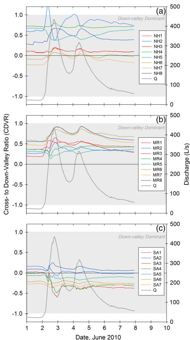
Figure 7. WS01 cross- to down-valley hydraulic gradient ratio (CDVR) for the 1–8 June storm period, for (a) the near-hillslope zones, (b) the middle riparian zones, and (c) the stream adjacent zones. The grey band indicates the region of down-valley dominance (i.e., |\text{CDVR}| < 1 ). Tick marks are displayed at 00:00 on the day labeled.
