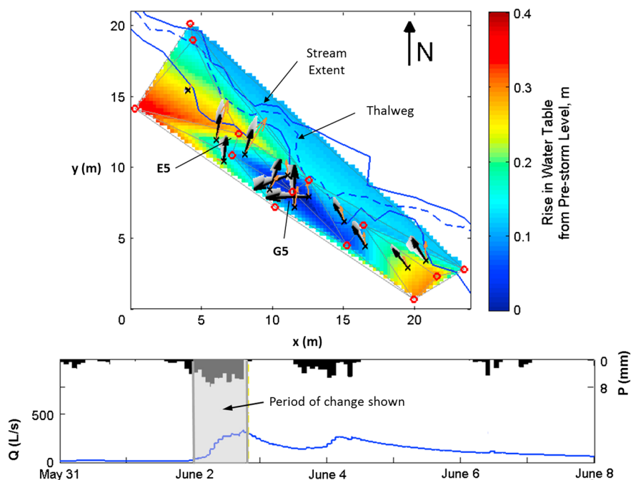
Figure 10. Time-lapsed image of the riparian hydraulic gradient storm response in WS03. Red circles indicate locations of water level measurement. Hydraulic gradient arrows (originating at x 's) are plotted such that the arrow color transitions from light grey to black as time progresses over the storm response period. Brown arrows show the surface topographic gradients at the centroid of each element. The colored background indicates the rise in water level from the pre-storm level, to show how water levels rose to produce the observed gradient changes. Flow is from bottom right to top left. Tick marks are displayed at 00:00 on the day labeled. Hydrograph ( Q ) in blue and hyetograph ( P ) in black are presented in the bottom panel.
