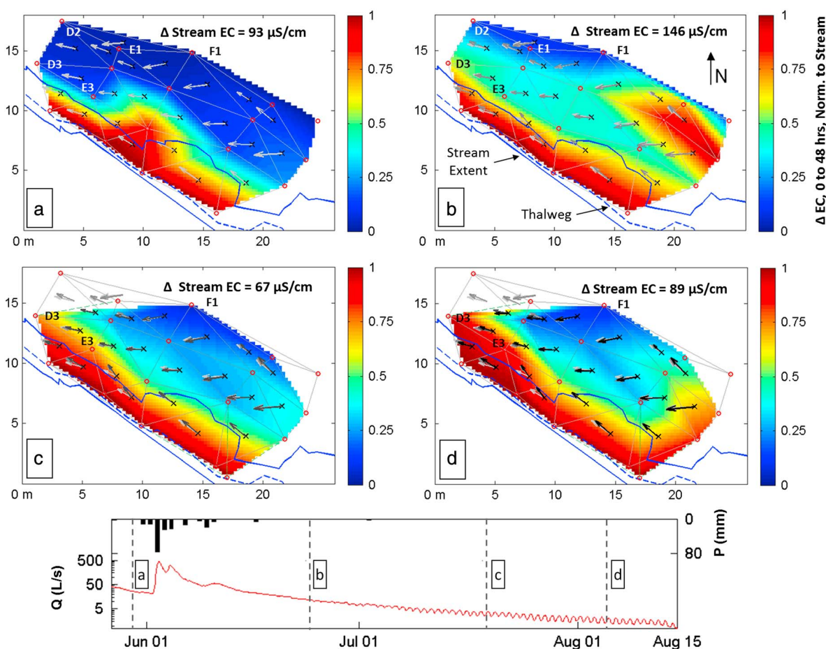
Figure 13. Change in EC in the WS01 riparian zone from 0th to 48th h of four 48 h constant-rate salt tracer injections, normalized to the change in stream EC, set to 1. Gradients at each time step are displayed as arrows that grow darker in color and stack above the earlier arrows as time advances. The colored area diminishes in size as less data becomes available due to wells drying out. The salt tracer was injected about 40 m above the upstream-most well transect. Flow is from bottom right to top left. Hydrograph ( Q ) in red and hyetograph ( P ) in black are presented in the bottom panel.
