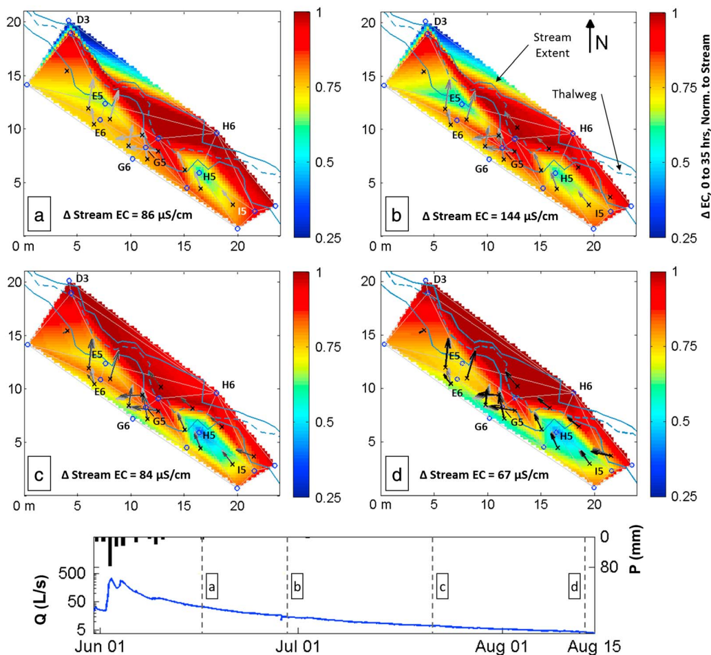
Figure 14. Change in EC in the WS03 riparian zone from 0th to 35th h of four 48 h constant-rate salt tracer injections, normalized to the change in stream EC, set to 1. Gradients at each time step are displayed as arrows that grow darker in color and stack above the earlier arrows as time advances. Blue circles denote wells. The salt tracer was injected about 40 m above the upstream-most well transect. Note that the color bar axis limits are from 0.25 to 1, unlike those in Figure 8 for WS01. Flow is from bottom right to top left. Hydrograph ( Q ) in blue and hyetograph ( P ) in black are presented in the bottom panel.
