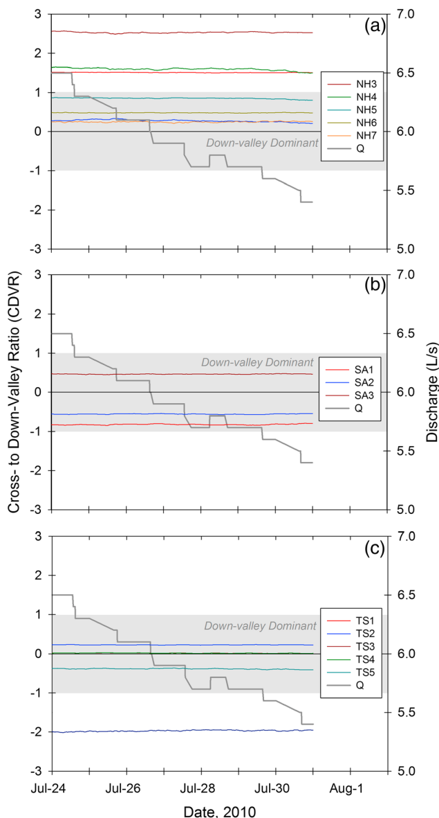
Figure 12. WS01 cross- to down-valley hydraulic gradient ratio (CDVR) for the period from 24 to 31 July when stream flow demonstrated a pronounced diurnal fluctuation due to evapotranspiration within the catchment, for (a) the near hillslope zone, (b) the stream adjacent zone, and (c) the through stream zone. Tick marks are displayed at 00:00 on the day labeled.
