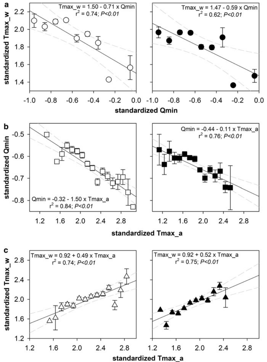
Fig. 4 Standardized magnitudes of stream temperature maxima ( T_{\max\_w} ) versus low flow minima ( Q_{\min} ) versus air temperature maxima ( T_{\max\_a} ) for 1-d ( open symbols ) and 7-d MA events ( filled symbols ). All symbols represent mean \pm SE of all available sites, grouped every 5 years. Standardized magnitude was grouped into classes of 0.1 units. Dashed lines represent 95% confidence intervals for the regression line. a Magnitude of T_{\max\_w} versus magnitude of the Q_{\min} for 1-d and 7-d MA events. b Magnitude of Q_{\min} versus magnitude of the T_{\max\_a} for 1-d and 7-d MA. c Magnitude of T_{\max\_w} versus magnitude of the T_{\max\_a} for 1-d and 7-d MA events
