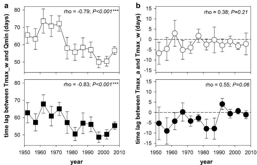
Fig. 3 Time lag (as number of days) between annual hydro-climatic events. a Number of days that annual stream temperature maxima ( T_{\max_w} ) preceded annual stream flow minima ( Q_{\min} ) for 1-d (open square) and 7-d MA (filled square) events. b Number of days that annual stream temperature maxima ( T_{\max_w} ) preceded annual air temperature maxima
