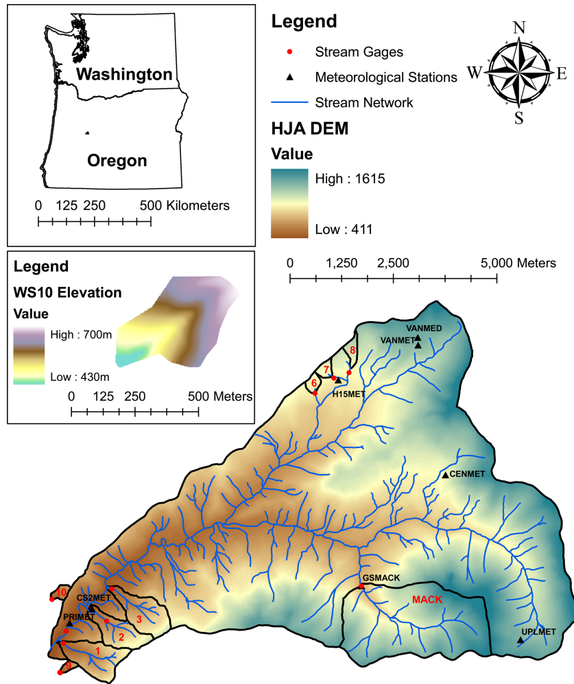
Figure 1. The study site is the WS10 of the HJA located in the western Cascade Range of Oregon. The red dots represent the locations of the stream gages. The black triangles represent the locations of the meteorological stations.
