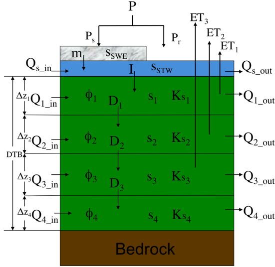
Figure A2. The soil column hydrological framework consists of a four-layered soil column, a standing water layer, and a snow layer. DTB is the soil column depth to bedrock. \Delta z_i , Ks_i , \phi_i , and s_i are the thickness, the saturated hydraulic conductivity, the soil porosity, and the soil water storage of layer i , respectively; P , P_s , and P_r are the precipitation, snow, and rain, respectively; m is the snowmelt, and s_{SWE} is the snow water equivalent depth; I is the infiltration, and s_{STW} is the standing water amount; Q_s is the surface runoff; and Q_i , D_i , and ET_i are the subsurface runoff, the drainage and the ET of layer i , respectively.
