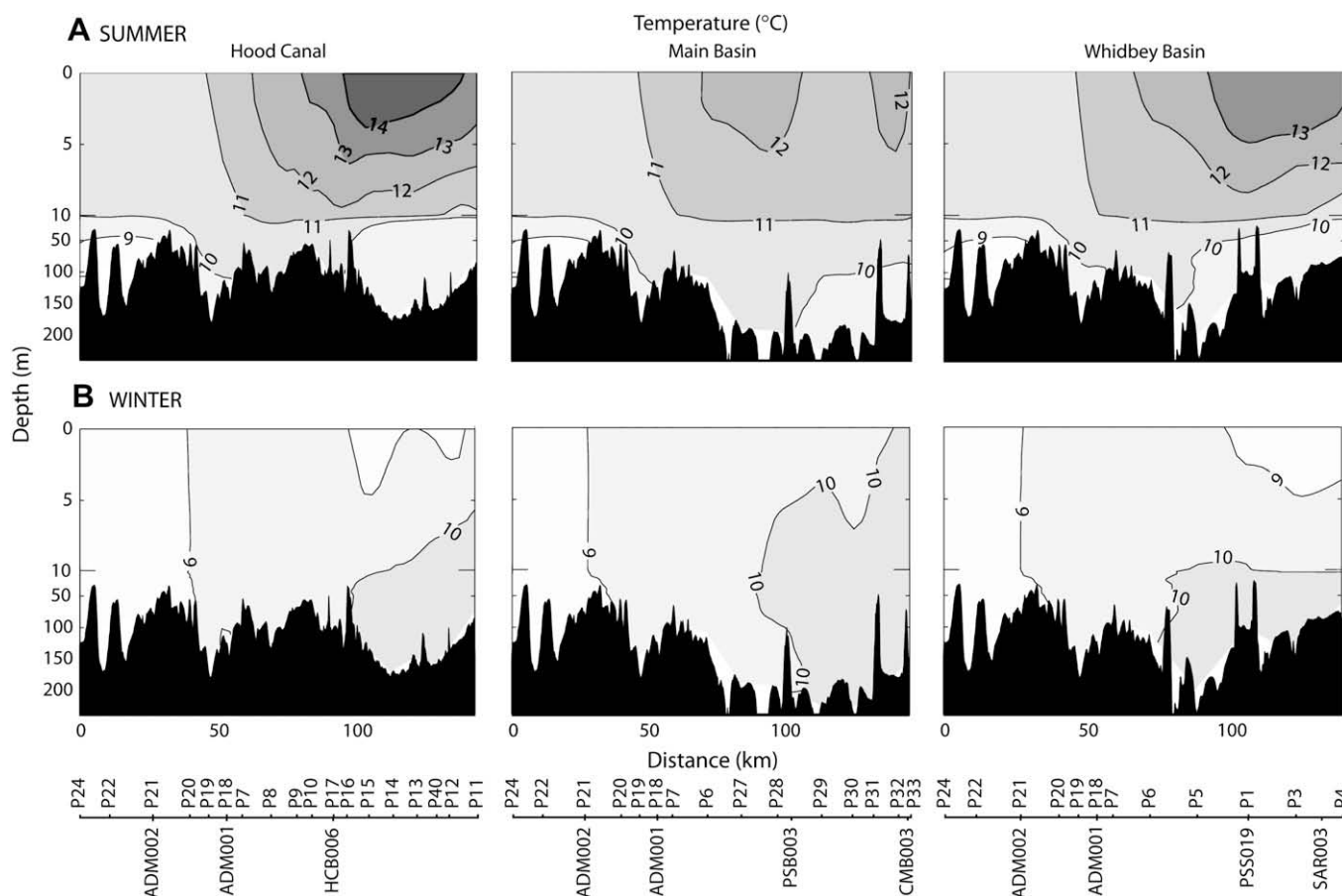
Fig. 5. Mean of summer (panel A) and winter (panel B) temperature (°C) along Puget Sound Regional Synthesis Model transects in Main Basin, Whidbey Basin, and Hood Canal from 1998 to 2003. Note that the upper 10 m of the water column is plotted on an enlarged depth scale.
