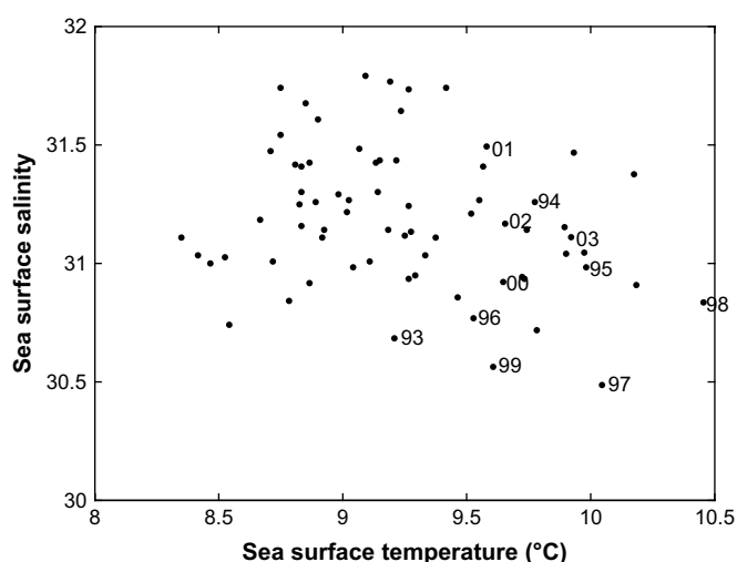
Fig. 8. Annual mean sea surface temperature and salinity at Race Rocks from 1937 to 2002. Values representing the time period examined in this study from 1993 to 2002 are labeled. Figure modified from Moore et al. (2008). Copyright (2008) by the American Society of Limnology and Oceanography, Inc.
