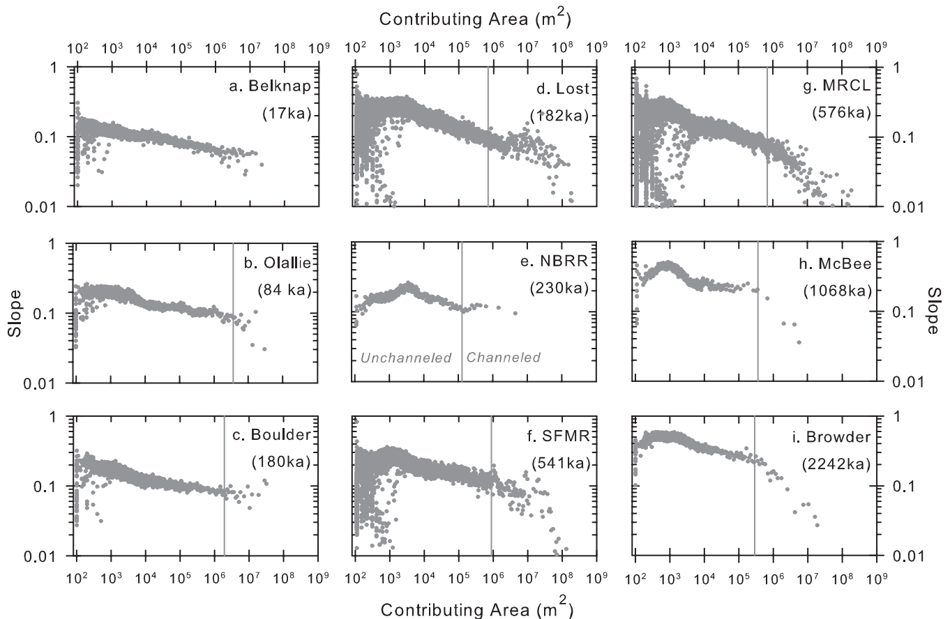
Figure 6. Slope–area relationships for High Cascades study watersheds. The vertical bar represents the average contributing area of channel heads in the watershed, with points to the left of the bar representing unchanneled areas and points to the right of the bar representing the stream network. There are no channels in the Belknap watershed.
