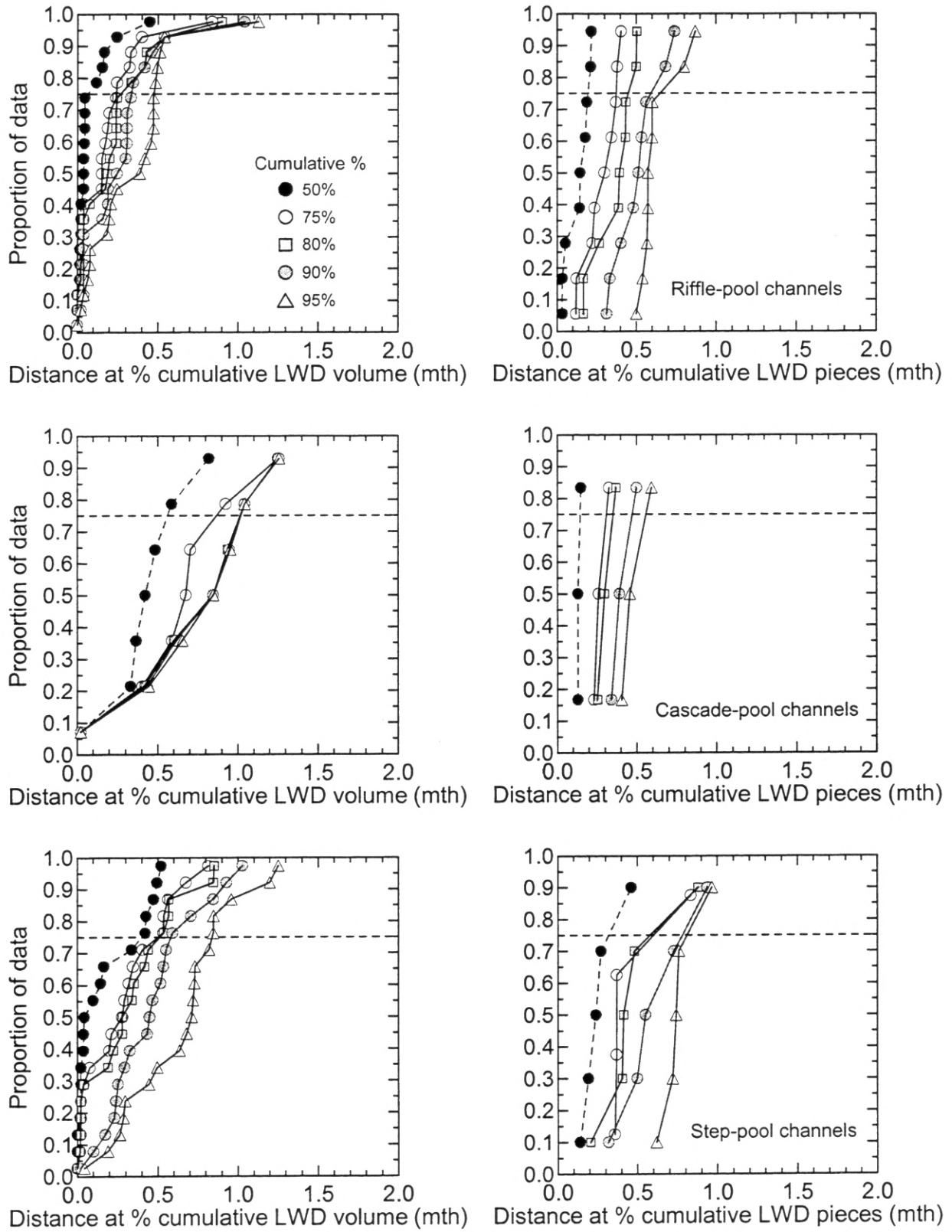
Fig. 2b. Quantile plots of the source distances (units of mean tree heights) within which specified proportions of the cumulative inputs of large woody debris (LWD) volume or numbers originated at different channel types.
