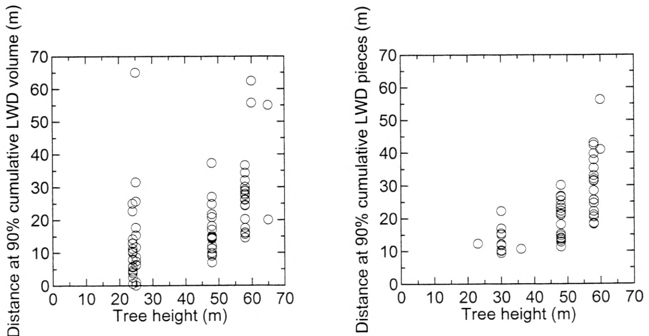
Fig. A1. The lateral distance from the stream channel edge within which 90% of the cumulative volume (left panel, N = 83) or numbers (right panel, N = 53) of large woody debris pieces originated, as a function of the reported tree height of the riparian forest. Where tree height was reported as a mean for many sites, all sites have been assigned the same value.
