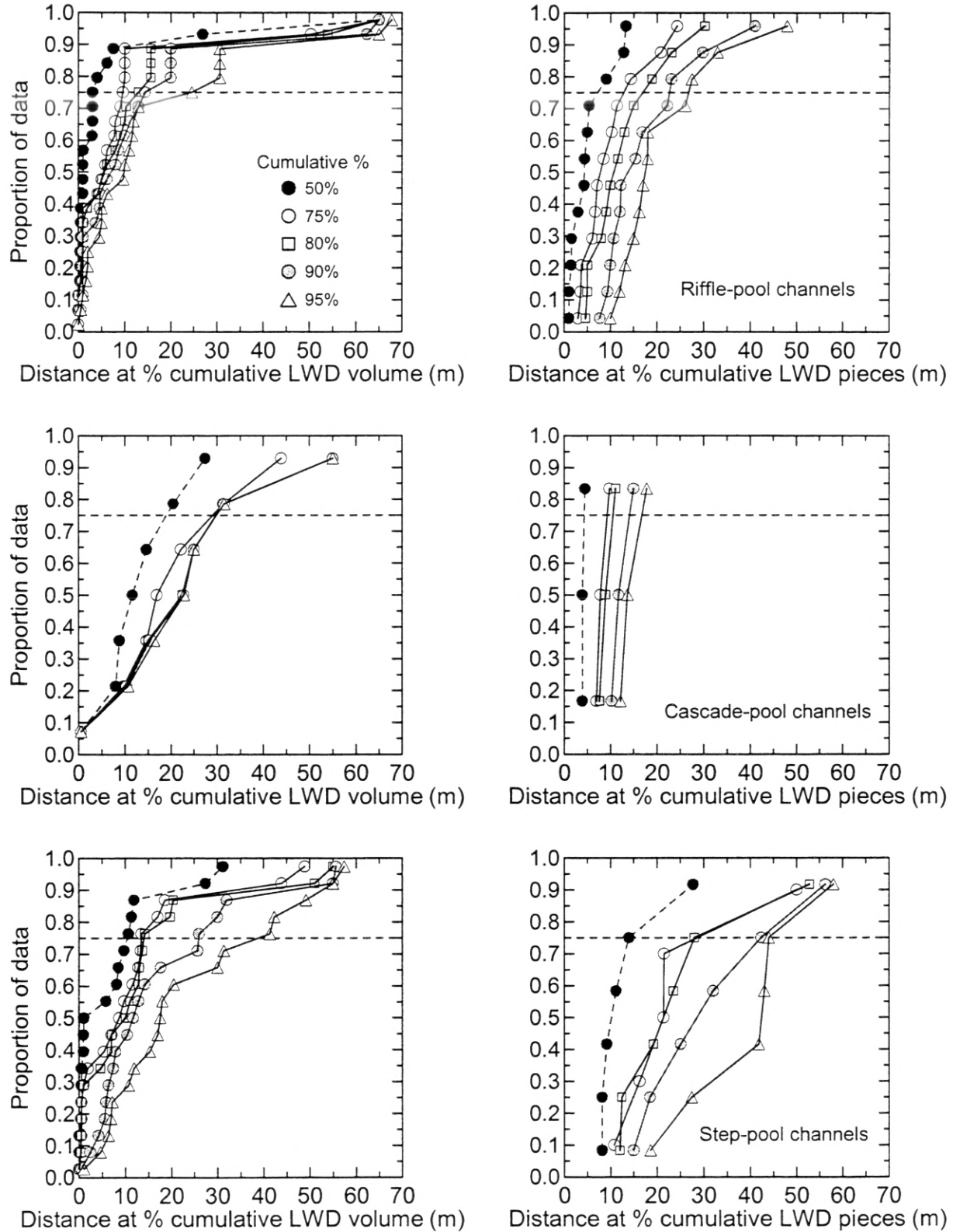
Fig. 2a. Quantile plots of the source distances (m) within which specified proportions of the cumulative inputs by volume (left panel) or number (right) of large woody debris (LWD) pieces originated at different channel types.
