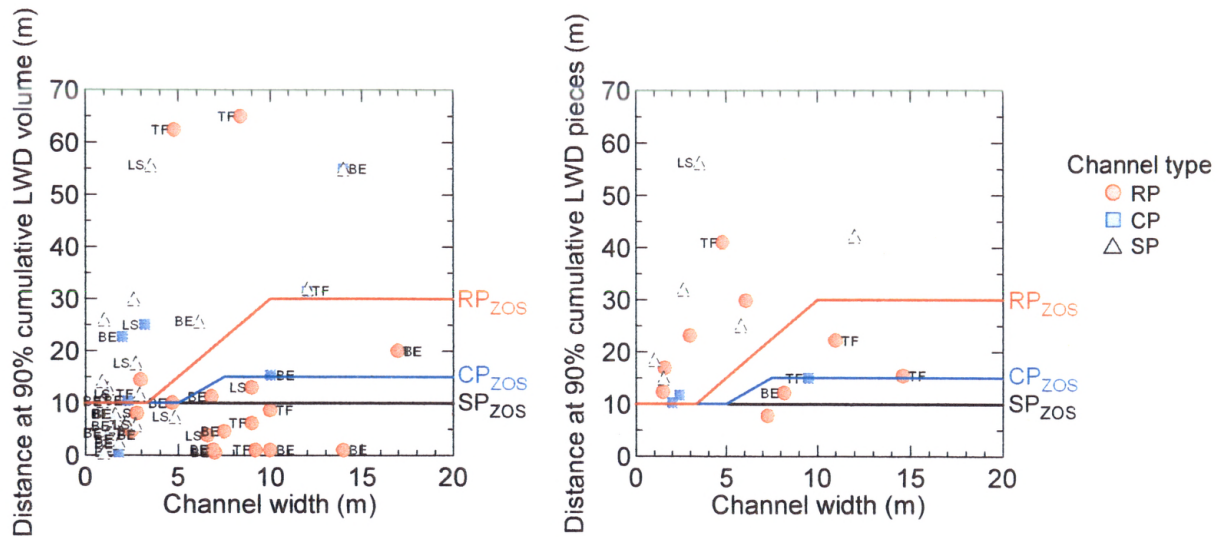
Fig. 5. Effects of channel width, channel type, and dominant delivery mechanism on the source distance within which 90% of the volume (left panel) and number (right panel) of large woody debris (LWD) pieces originate. Channel types are riffle-pool (RP), cascade-pool (CP), and step-pool (SP). LWD delivery mechanisms are bank erosion (BE), land slides (LS), and tree fall (TF). Lines indicate the “zone of sensitivity” defined for different channel types and widths under the BC Riparian Area Regulations (see Table 1 for details).
