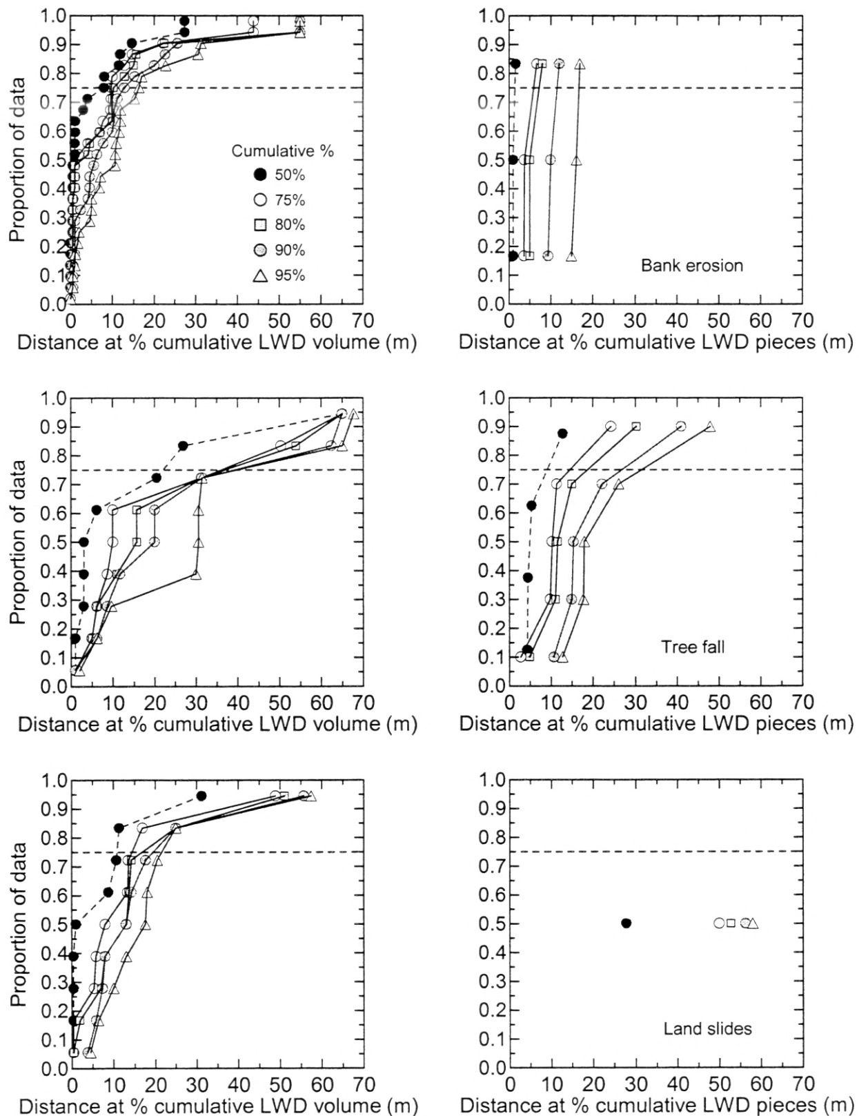
Fig. 3a. Quantile plots of the source distances (m) within which specified proportions of the cumulative inputs of large woody debris (LWD) volume or numbers originated for different dominant input mechanisms.
