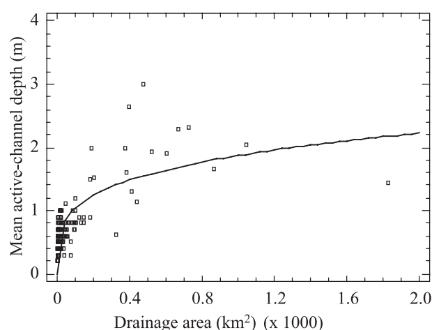
FIGURE 10. Relationship Between Field-Measured Mean Active-Channel Depth ( H_a ) and Modeled Drainage Area ( D ) ( H_a = 0.328 \times D^{0.252} ) ( R^2 = 0.64 ; df = 273 ; p < 0.0001 ).
