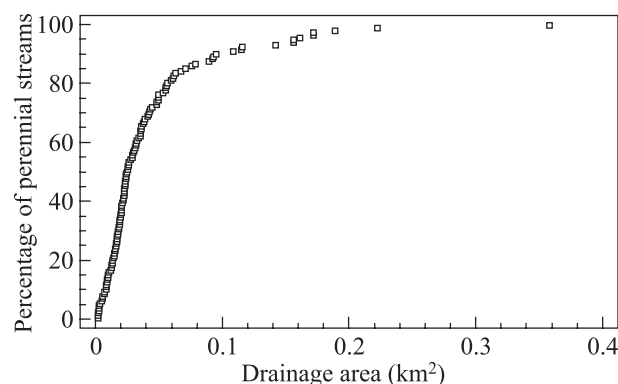
FIGURE 6. Cumulative Distribution Function of Drainage Areas Corresponding to the Upper Limit of Field-Determined Perennial Flow for Streams in the Siuslaw National Forest Dataset.
