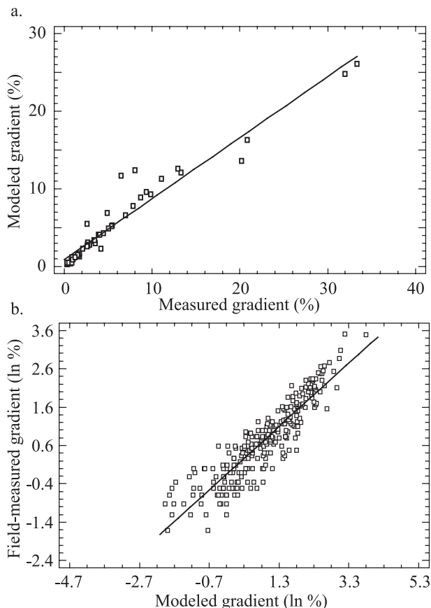
FIGURE 7. Modeled Channel Gradients ( S_m ) Regressed With (a) Map-Measured Gradients and (b) Field-Measured Gradients ( S_f ) ( \ln(S_f) = 0.02 + 0.83 \times \ln(S_m) ( R^2 = 0.82 ; df = 251 ; p < 0.0001 ).
