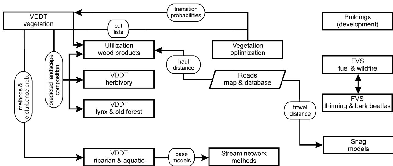
Fig. 1. Relation between INLAS modules (boxes) showing types of information (ovals) transferred between modules. Although the description of the roads module (parallelogram) is published elsewhere (Aitken and Hayes, in press ), information on the road network was used to estimate haul distances for wood products removed from the forest and for estimating travel distances to access areas for fuel wood cutting.
