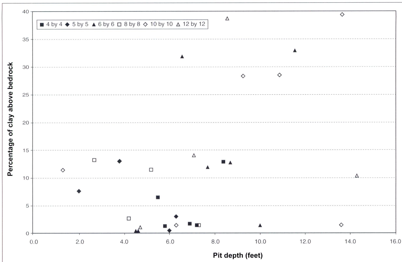
Figure 20—Percentage of clay within 6 in of bedrock versus depth to bedrock.
