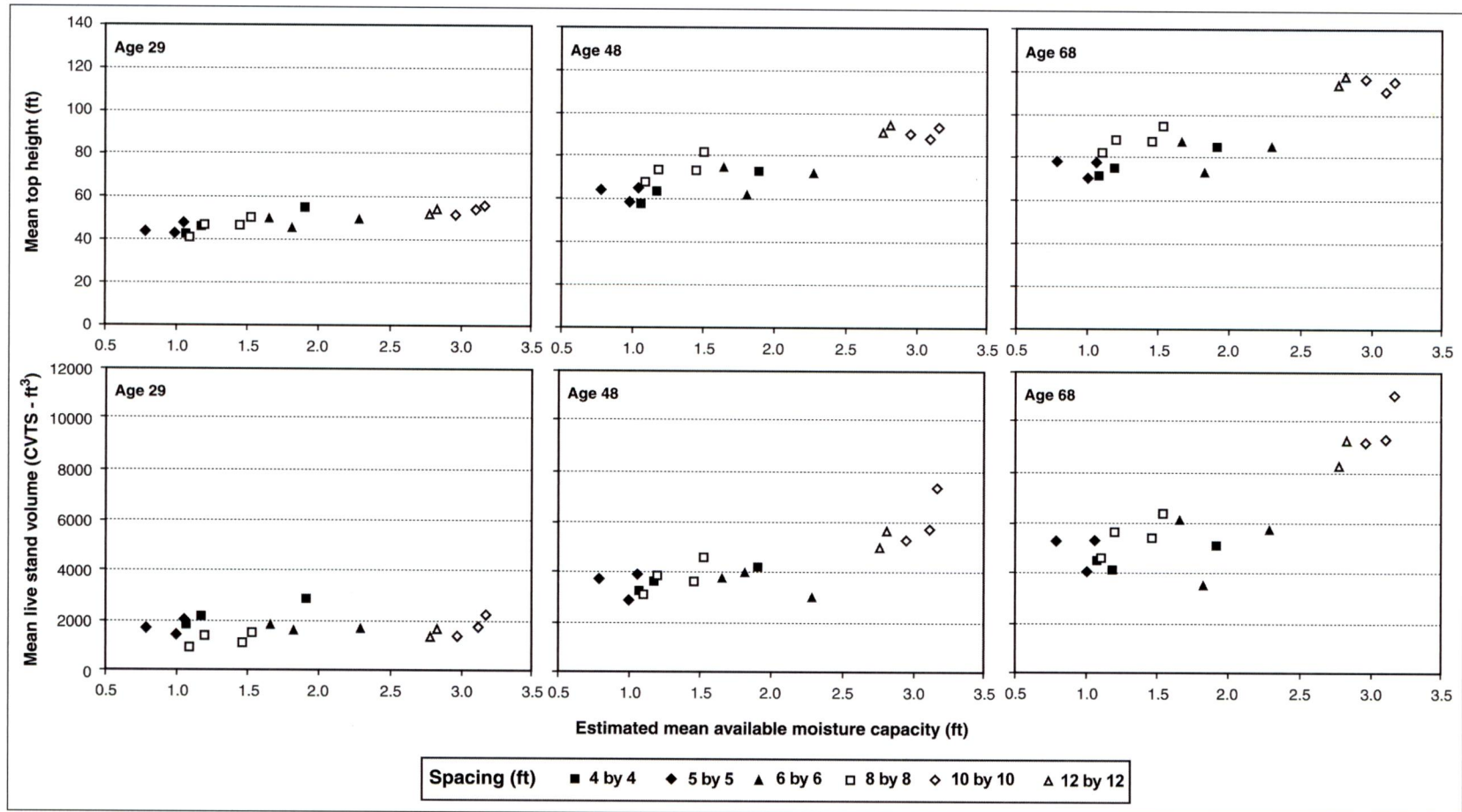
Figure 17—Mean top height (H40) and live stand volume (CVTS) related to estimated mean available water capacity at tree ages 29, 48, and 68 years.
