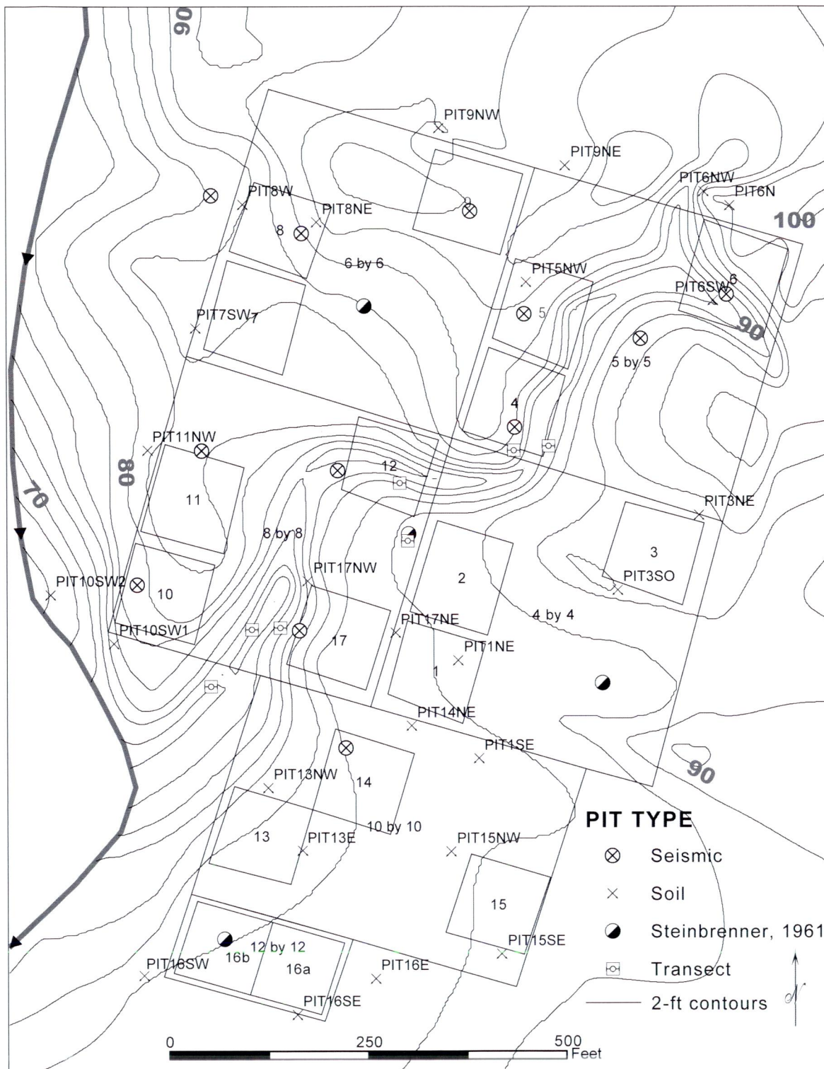
Figure 4—Location of soil pits and seismic measurements.
