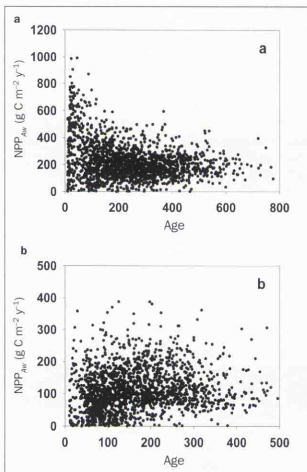
Figure 5. Aboveground wood net primary production ( NPP_{Aw} ; grams of carbon per square meter per year) and stand age (years) at permanent plots managed by the USDA (US Department of Agriculture) Forest Service's Forest Inventory and Analysis Program in two ecozones, (a) the western Cascades and (b) the eastern Cascades. Adapted from Law and colleagues (forthcoming).
