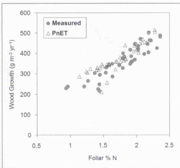
Figure 2. The relationship between foliar nitrogen (N) concentration (as a percentage of leaf mass) and wood growth (in grams of carbon per square meter per year) for 38 growth-inventory plots at the Bartlett Experimental Forest in north-central New Hampshire. Shaded symbols show the field-measured relationship; open symbols show the predicted relationship, generated by combining remotely sensed canopy nitrogen estimates (from the Airborne Visible/Infrared Imaging Spectrometer, or AVIRIS) with the PnET ecosystem model.
