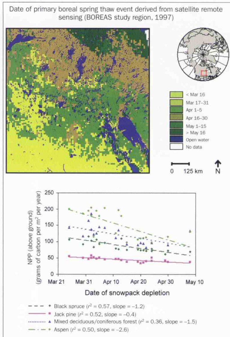
Figure 3. Satellite remote sensing (top) of the 1997 primary spring thaw event for the Boreal Ecosystem-Atmosphere Study (BOREAS) study region, derived from temporal classification of daily radar backscatter information from the NASA (National Aeronautics and Space Administration) Scatterometer, or NSCAT. The dates in the legend represent the interval during which thaw occurred. Graph (bottom panel) shows the relationship between measurements of aboveground net primary production (NPP) for different forest types by year within the study region and corresponding estimates of snowpack depletion, a surrogate measure of spring thaw timing. Years with an early spring tend to promote greater annual NPP, whereas years with a delayed spring promote the opposite response. Adapted from Kimball and colleagues (2000, forthcoming).
