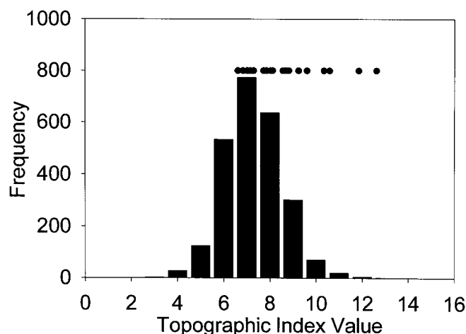
Figure 2. Topographic index distribution of Dry Creek. Dots represent index values of well locations
