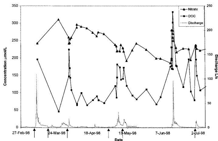
Figure 3. Discharge and stream chemistry. Arrows indicate time of sampling
