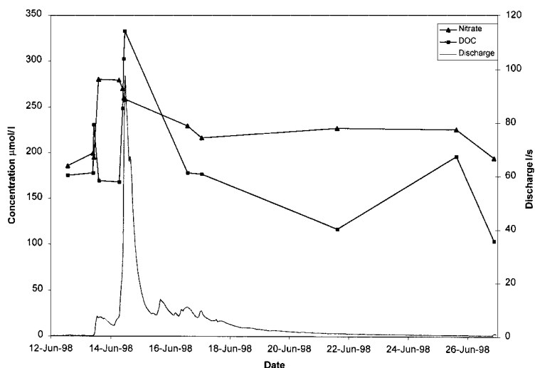
Figure 4. Stream discharge and chemistry showing flushing effects of a large storm
