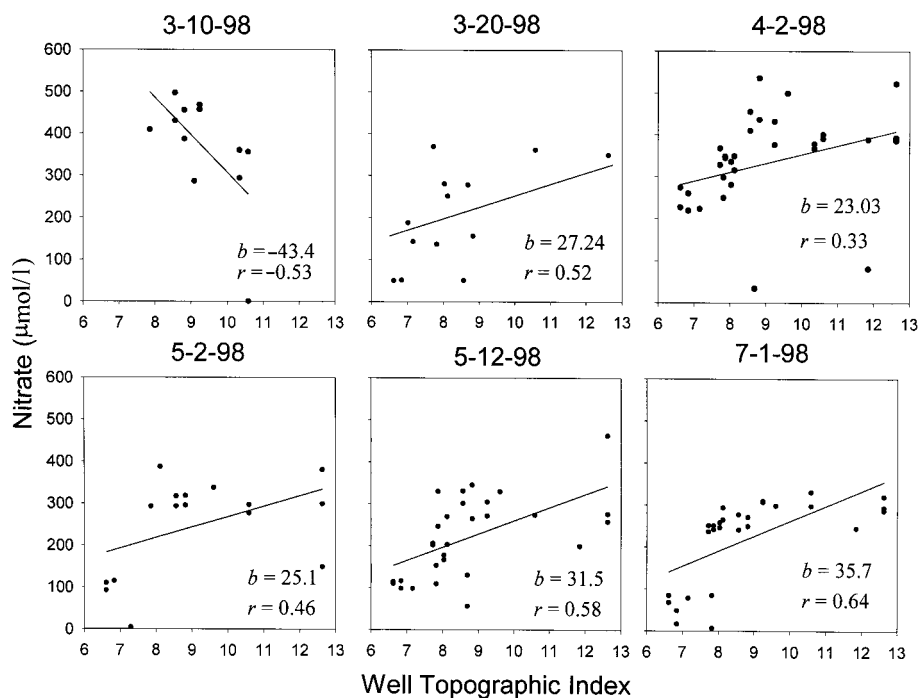
Figure 5. Nitrate–TI relationship for all six storms sampled
