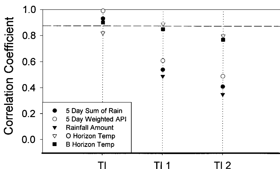
Figure 8. Correlation coefficients for the controls on the strength of the topography–chemistry relationship. Dashed horizontal lines represent confidence intervals at the 5% level
