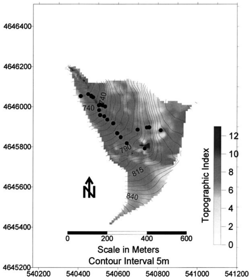
Figure 1. Topographic index map of Dry Creek. Dots represent piezometer locations. Axes are UTM metres
