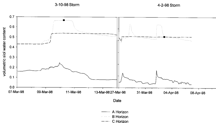
Figure 6. Soil moisture for 3-10-98 and 4-2-98. Dot indicates time of sample
