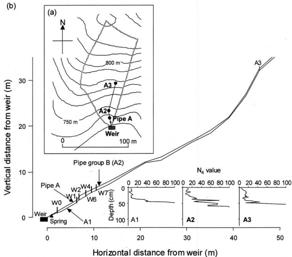
Figure 2. (a) Topographic map of the Toinotani watershed with a 10 m contour interval. (b) Longitudinal axis of the concave slope (line Weir-A3, as noted in Figure 2a). The profiles of the N_4 penetrometer values are shown in the inset graph.
