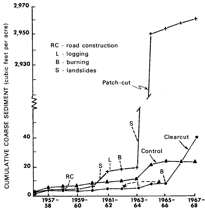
Figure 5.-Accumulated volume of coarse sediment trapped in catch basins.
