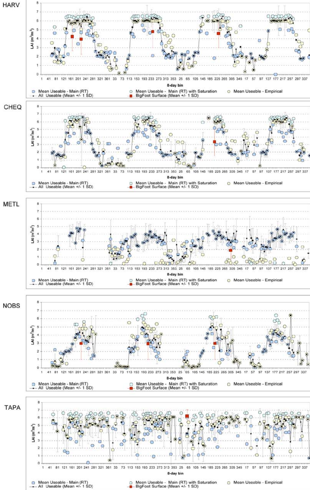
Fig. 6. (Continued). MODIS LAI estimates by algorithm pathway and across pathways between 2000 and 2003 for the 7 \text{ km} \times 7 \text{ km} areas of the nine study sites. See [6] for a description of why BigFoot LAI values in this figure and Table II are different.
