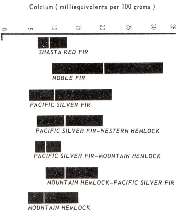
Figure 5.--Amount of exchangeable calcium in forest floors under seven forest types. (The horizontal line is the average for the type, and the length of the bar represents the range.)
