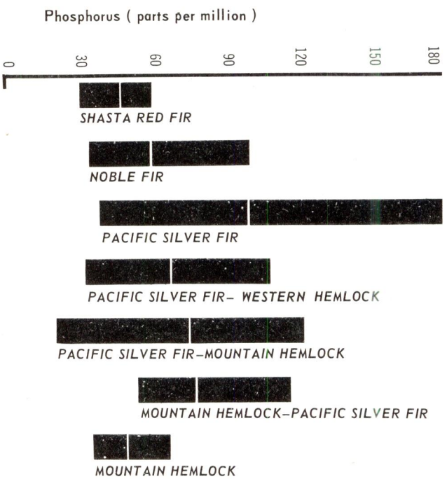
Figure 4.--Amount of available phosphorus in forest floors under seven forest types. (The horizontal line is the average for the type, and the length of the bar represents the range.)
