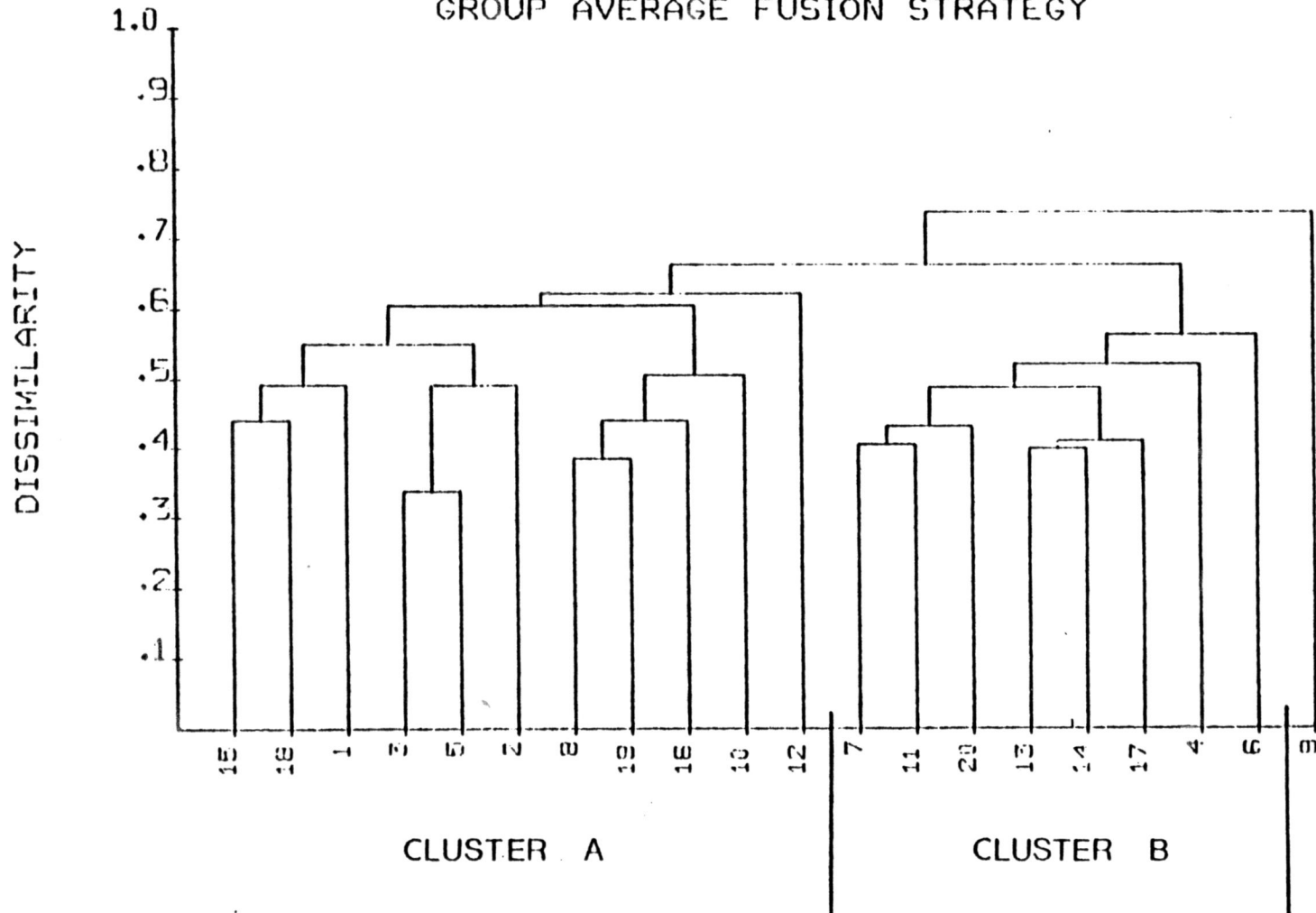
Figure 6. Hierarchical agglomerative clustering of Fraxinus latifolia plots.
