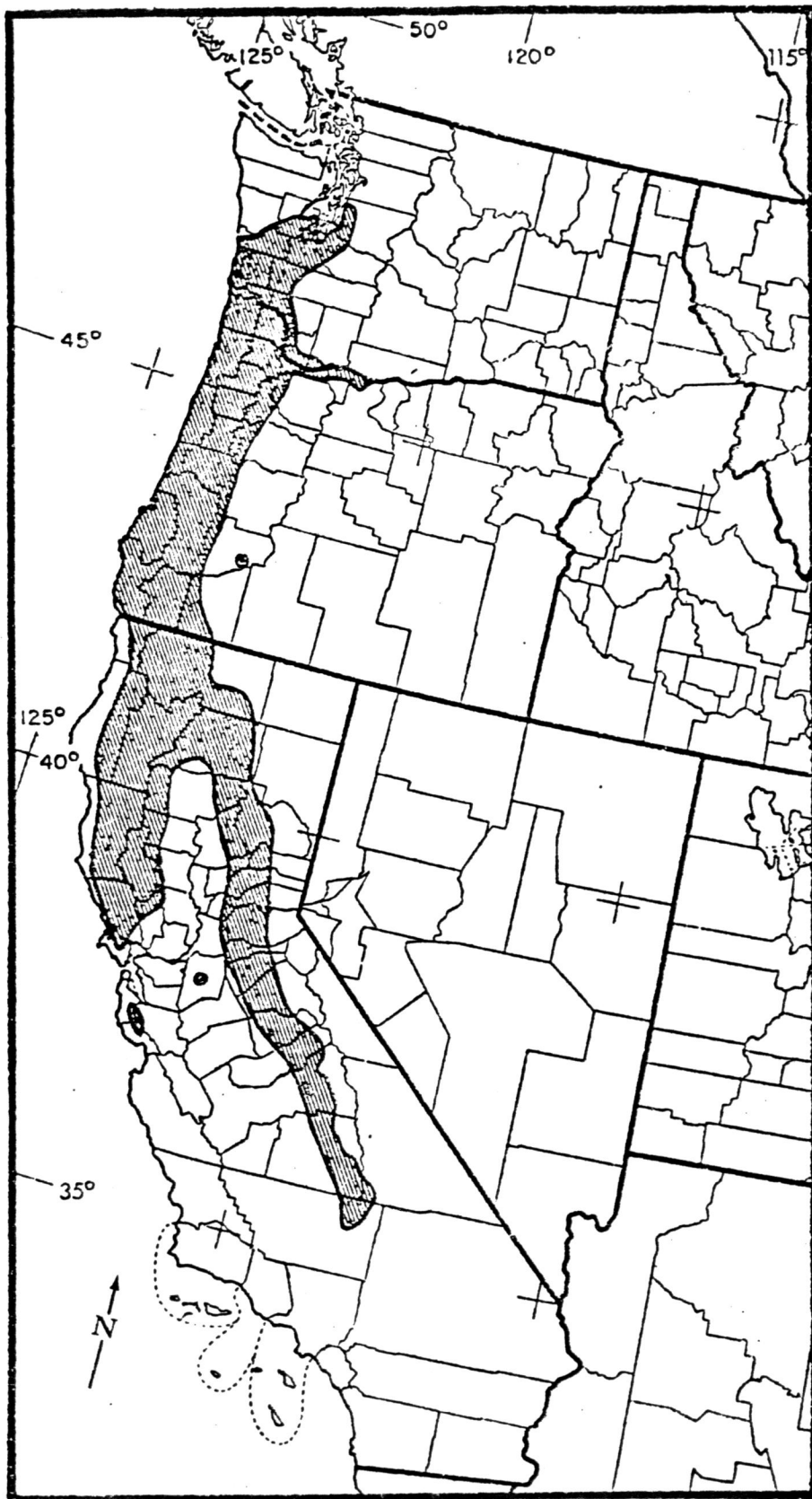
Figure 1. Natural range of Fraxinus latifolia Benth. from Little (1971).
