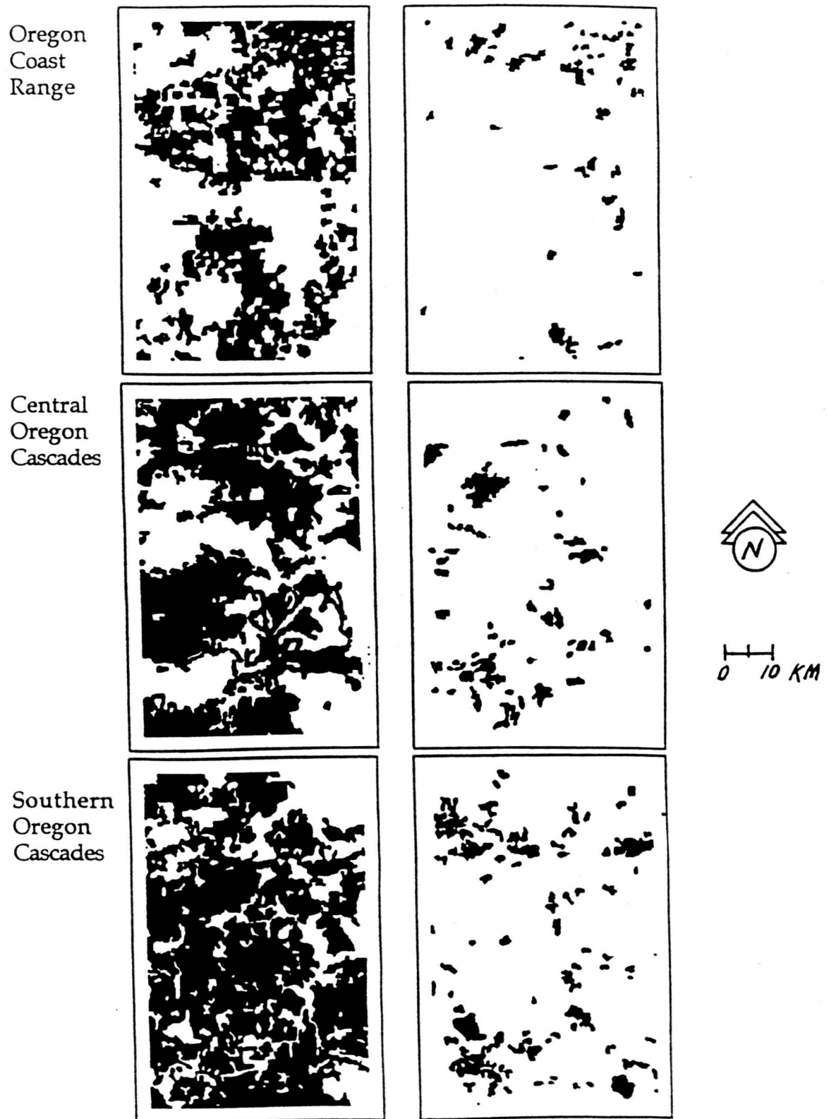
Figure 3.3 Pre-logging spatial pattern of old growth conifer (left in black) and recent fire patches (right in black).
