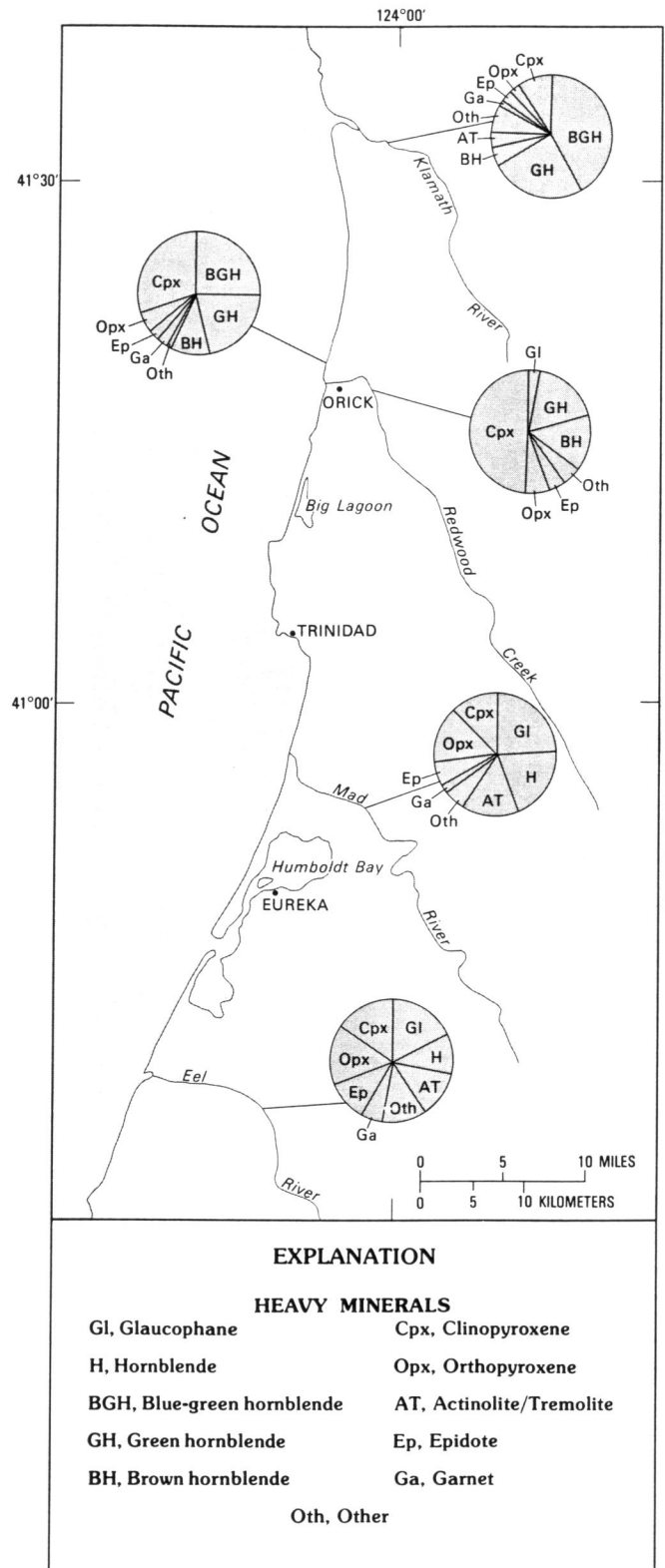
FIGURE 11.—Heavy-mineral analyses of northern California river sands and of the beach sand near the mouth of Redwood Creek. Klamath River data from Kulm and others (1968); Mad and Eel River data from Bodin (1982); and Redwood Creek and beach data from Curt Peterson (written commun., 1982).
