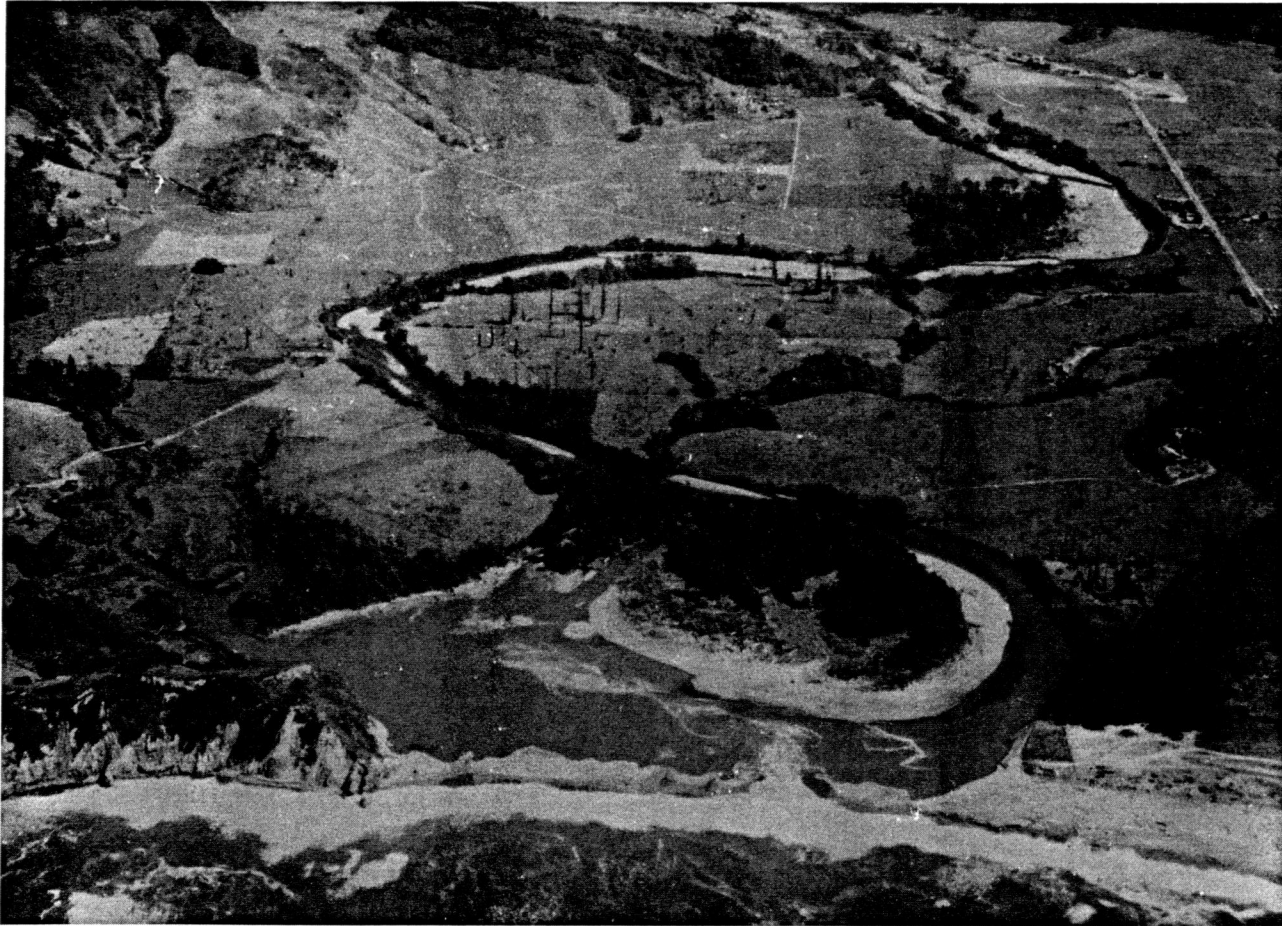
FIGURE 3.—Oblique aerial photograph of mouth of Redwood Creek, September 1948.
