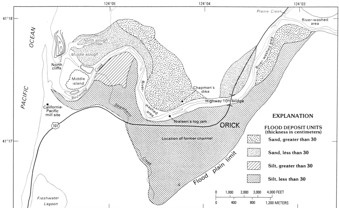
FIGURE 1.—Redwood Creek flood plain showing 1964 flood deposits and selected cultural features. This map shows the configuration of the mouth of Redwood Creek 2 weeks after the 1964 flood. Flood deposit units are from McLaughlin and Harradine (1965).
