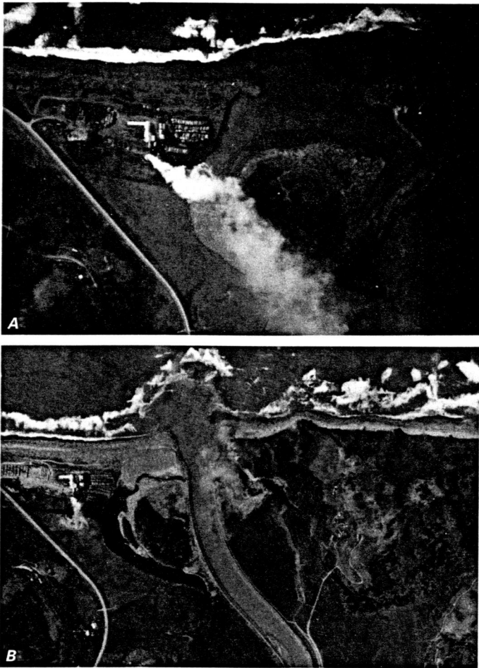
FIGURE 10.—Aerial photographs showing extent of scour of beach berm during major floods. A, January 13, 1965, following flood of December 18–24, 1964. B, March 7, 1972, following flood of March 1–4, 1972.
