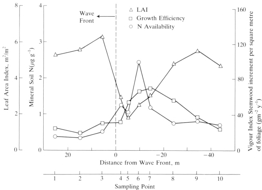
Figure 1. A transect on either side of a dieback zone (zero point) in a subalpine mountain hemlock forest. Leaf Area Index (LAI) decreases abruptly as the old growth forest is killed (0 to -10 m behind wave front). As a new forest is re-established, the canopy leaf area gradually increases again (-20 to -40 m). In conjunction with the death of the old forest, the young trees are provided more light and available nitrogen, the latter assessed by in situ incubation at 15-30 cm (Matson and Boone, 1984). As a result, tree vigour or growth efficiency initially improves significantly, but later decreases as the canopy again closes and nitrogen also becomes less available. We interpret increased tree vigour with resistance to the well distributed pathogen, Phellinus weirii and reduced vigour with susceptibility.
