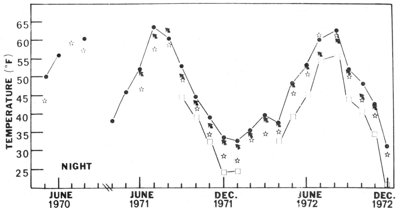
Fig. 2. Monthly mean night air temperatures at reference stands 1,3,7 and 14. Dots=RS1, Arrows=RS7, Stars=RS3 and Squares=RS14.
