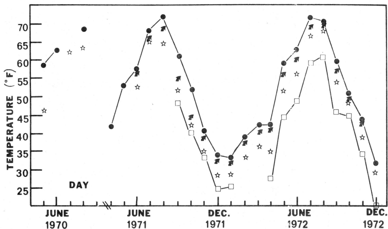
Fig. 3. Monthly mean day air temperatures at reference stands 1,3,7 and 14. Dots=RS1, Arrows=RS7, Stars=RS3, and Squares=RS14.
