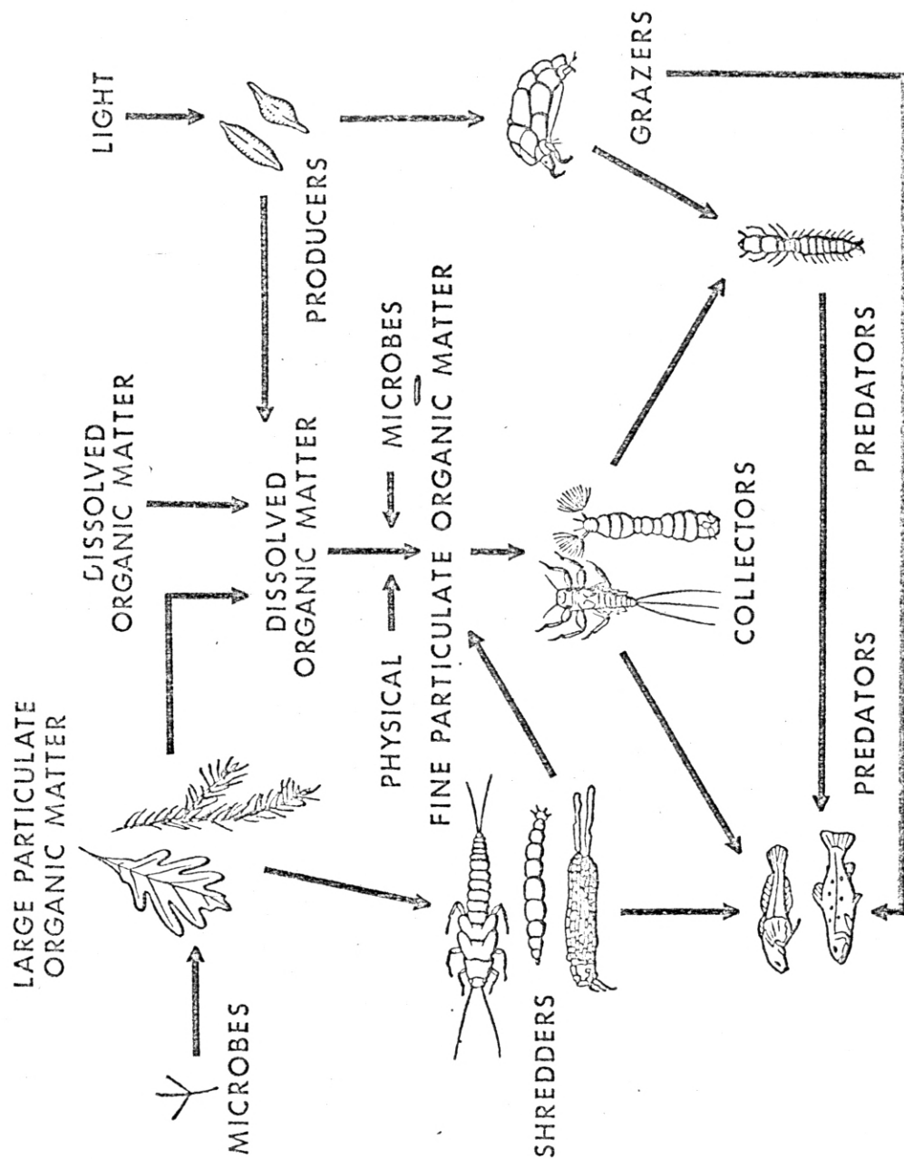
Figure 1. A simplified view of trophic relationships in a woodland stream community. Deciduous leaves, coniferous needles, and photosynthesis by diatoms are utilized, together with soil runoff, as representative of energy inputs to the system. Pteronarcys , Tipula , and Pycnopsycha are shown as typical shredders, Stenonema and Simulium as collectors, Glossosoma as a grazer, and Nigronia and the fish Cottus and Salmo as predators. Litter microbes are characterized by fungi (such as aquatic hyphomycetes) and fine particle microbes by bacteria.
