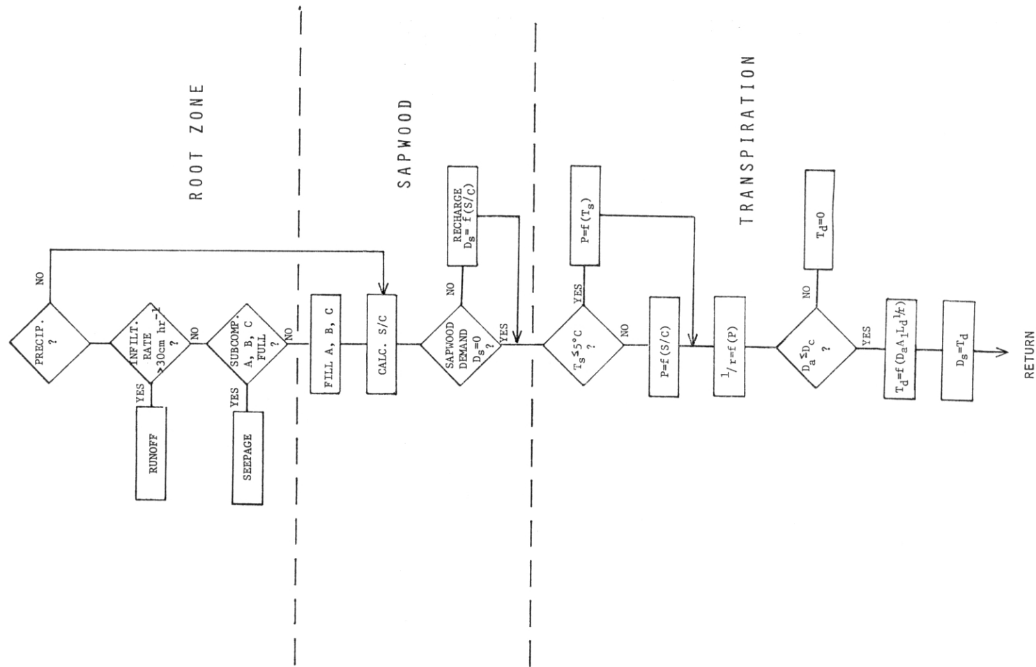
Fig. 5. Flow diagram of computer simulation model
