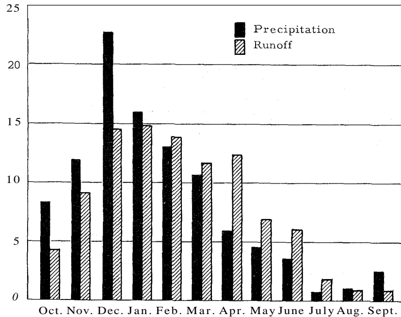
Average annual distribution of precipitation and runoff from the Lookout Creek drainage.
