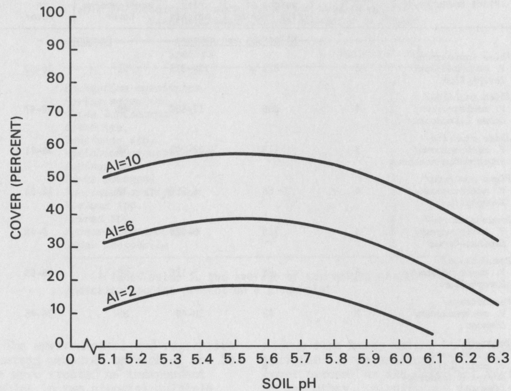
Figure 1.--Calculated relation of soil pH to Vaccinium membranaceum cover at three abundance indices (AI). Calculated from VMC\% = -1.302.79 + 5.0074(AI) + 475.815(pH) - 43.1596(pH^2) ; r^2 = 0.602 .
