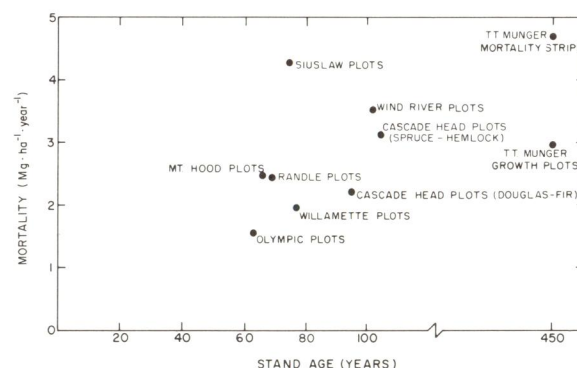
FIG. 4. Transfer to the forest floor resulting from tree mortality as a function of stand age (mortality and age averaged over the length of time each stand was studied).
