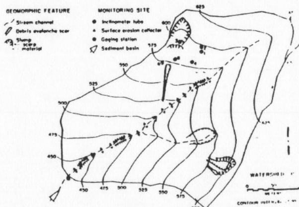
FIGURE 8.3 Geomorphic features and monitoring sites on watershed 10
