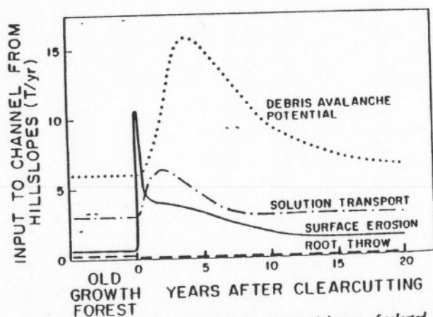
FIGURE 8.4 Hypothetical trajectories of potential rates of selected hillslope transfer processes after clearcutting of watershed 10.
