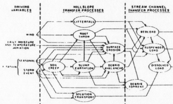
FIGURE 8.2 Relations among mass transfer processes and principal driving variables. Arrows indicate that one process influences another by supplying material for transfer or creating instability that culminates in the occurrence of the second process.
