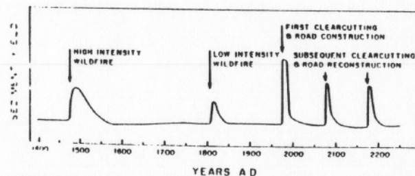
FIGURE 8.5 Hypothetical history of sediment yield in response to vegetation disturbances on watershed 10.
