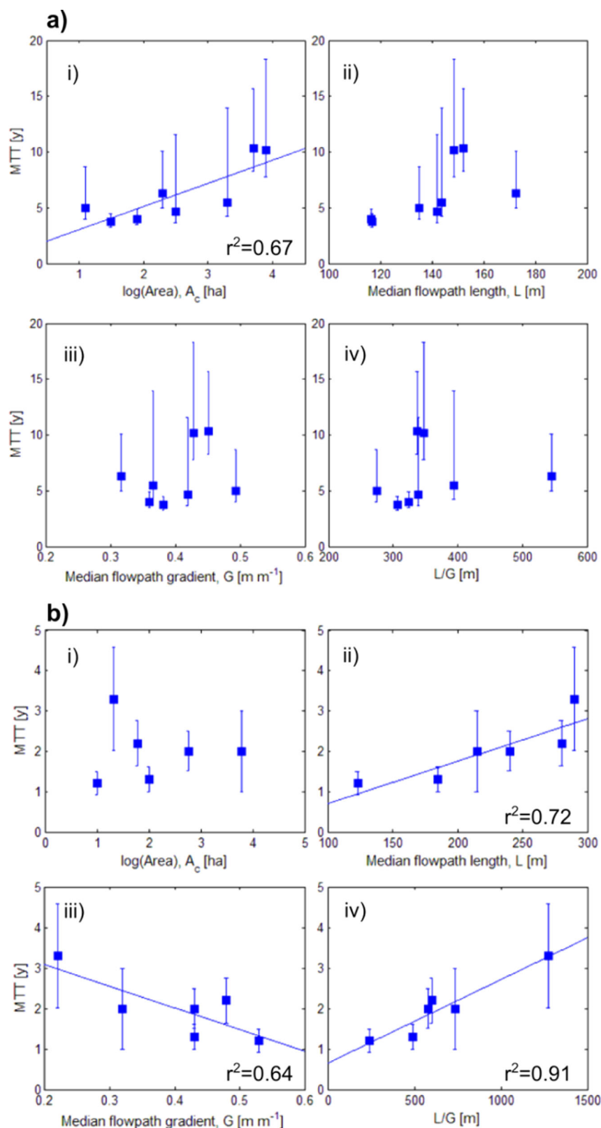
Figure 3. Mean transit time (MTT) as a function of the logarithm of (i) catchment area, (ii) median flow path length, (iii) median flow path gradient, and (iv) the ratio of median flow path length and flow path gradient for (a) the sedimentary Drift Creek catchments and (b) the volcanic HJ Andrews catchments.
