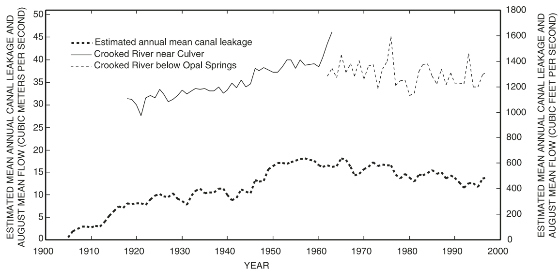
Figure 35. Hydrograph showing estimated canal losses north of Bend and August mean discharge of the Crooked River. Modified from Gannett et al. (2001).
