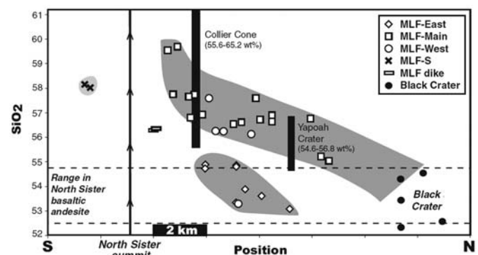
Figure 12. Illustration of the compositional variation of younger mafic lavas south of McKenzie Pass as a function of the distance from North Sister (from Schmidt and Grunder, 2009). This variation is interpreted to reflect the influence of a well-developed magma storage region beneath North Sister. MLF—Matthieu Lakes Fissure.
