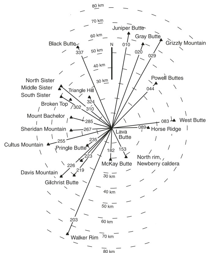
Figure 29. Compass wheel showing direction and distance to some geographic features visible from the top of Lava Butte. From Sherrod et al. (2002).
