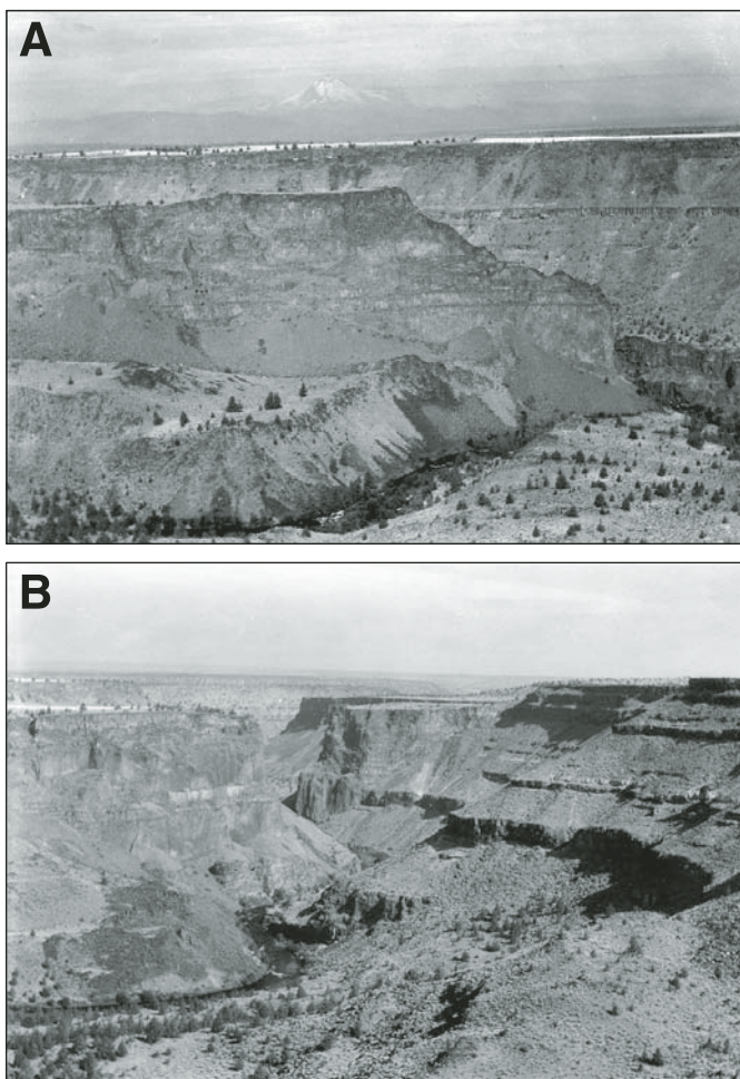
Figure 43. Photographs of the Crooked and Deschutes River canyons from the SE¼ sec. 35, T. 11 S., R. 12 E., taken by H.T. Stearns, August 1925, prior to inundation by Lake Billy Chinook (Stop 11). (A) View west across Crooked River canyon to The Island and, beyond it, the west rim of Deschutes River canyon. Deschutes-Crooked confluence is at right side of photograph in near ground, Mount Jefferson centered in background 45 km west-northwest. (B) View north (downstream) into Deschutes River canyon. Deschutes-Crooked confluence is at lower left edge of photograph. From Sherrod et al. (2002).
