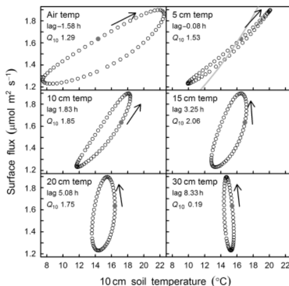
Fig. 1 Diel hysteresis between surface flux and soil temperature at several depths, and apparent Q_{10} values calculated from least squares regression (see text for details). Solid points show time = 12 h and arrows indicate the direction of hysteresis over time. Gray line represents the fitted mean that would produce an apparent Q_{10} equal to the input value of 2. D_T = 5 \times 10^{-7} m^2 s^{-1} (same data as bottom panel of Fig. 3). Negative lags indicate surface flux reaching a maximum before temperature whereas positive lags indicate temperature peaking first.
