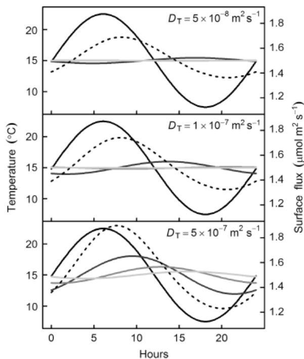
Fig. 3 Effect of thermal diffusivity, D_T , on soil temperatures at several depths (solid lines) and surface \text{CO}_2 flux (dotted line). Soil temperature depths from darkest to lightest are: soil surface, 10, 20, and 30 cm depth. See Table 1 for values of other input parameters.
