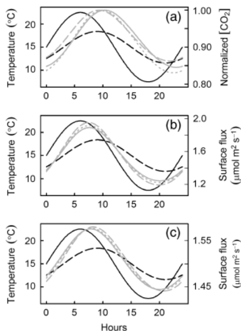
Fig. 5 Effect of \text{CO}_2 diffusivity on soil \text{CO}_2 concentrations and surface fluxes. (a) \text{CO}_2 concentration at 10 cm depth for three levels of D_{\text{CO}_2} : 5 \times 10^{-7} (solid gray), 1 \times 10^{-6} (dotted gray), 5 \times 10^{-6} (dashed gray). Air temperature (solid black) and 10 cm soil temperature (dashed black) are also shown. (b) Same as (a) except gray lines represent surface \text{CO}_2 flux. (c) Same as (b) except \text{CO}_2 production was uniformly distributed across soil profile, rather than decreasing exponentially with depth.
