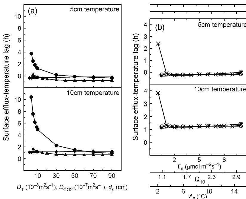
Fig. 4 Sensitivity of lag time to soil and environmental parameters. (a) Thermal diffusivity, D_T (●); CO_2 diffusivity, D_{CO_2} (◆); and exponential folding depth for CO_2 production, d_p (▲). (b) Basal total CO_2 production, \Gamma_0 (○); Q10 temperature sensitivity (×); and diel air temperature amplitude, A_0 (▼).
