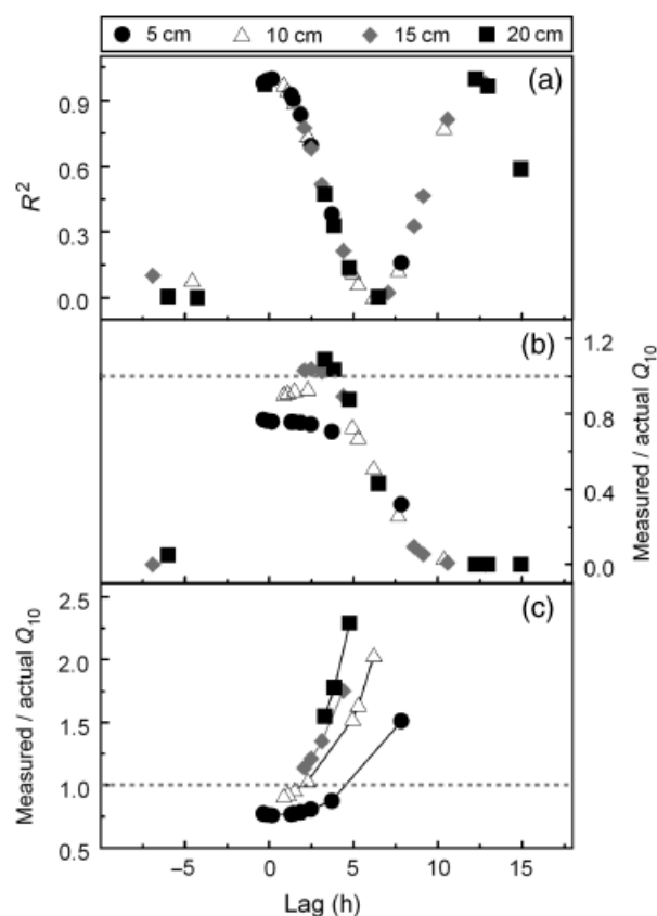
Fig. 2 Impact of phase lags on R^2 and apparent Q_{10} calculated from regressions of surface flux and soil temperature. (a) R^2 for regressions with soil temperature at reference depths of 5 cm (●), 10 cm (△), 15 cm (◆), and 20 cm (■). Lag time was varied by changing thermal diffusivity from 1 \times 10^{-8} to 9 \times 10^{-7} \text{ m}^2 \text{ s}^{-1} , as in Fig. 4a. (b) Apparent Q_{10} as a function of phase lag, normalized by the actual Q_{10} used to parameterize the model. (c) Same as (b), but surface flux data was shifted to be in-phase with soil temperature before calculating apparent Q_{10} . Apparent Q_{10} approached infinity with increasing phase lag, so only normalized values < 2.5 are shown for clarity.
