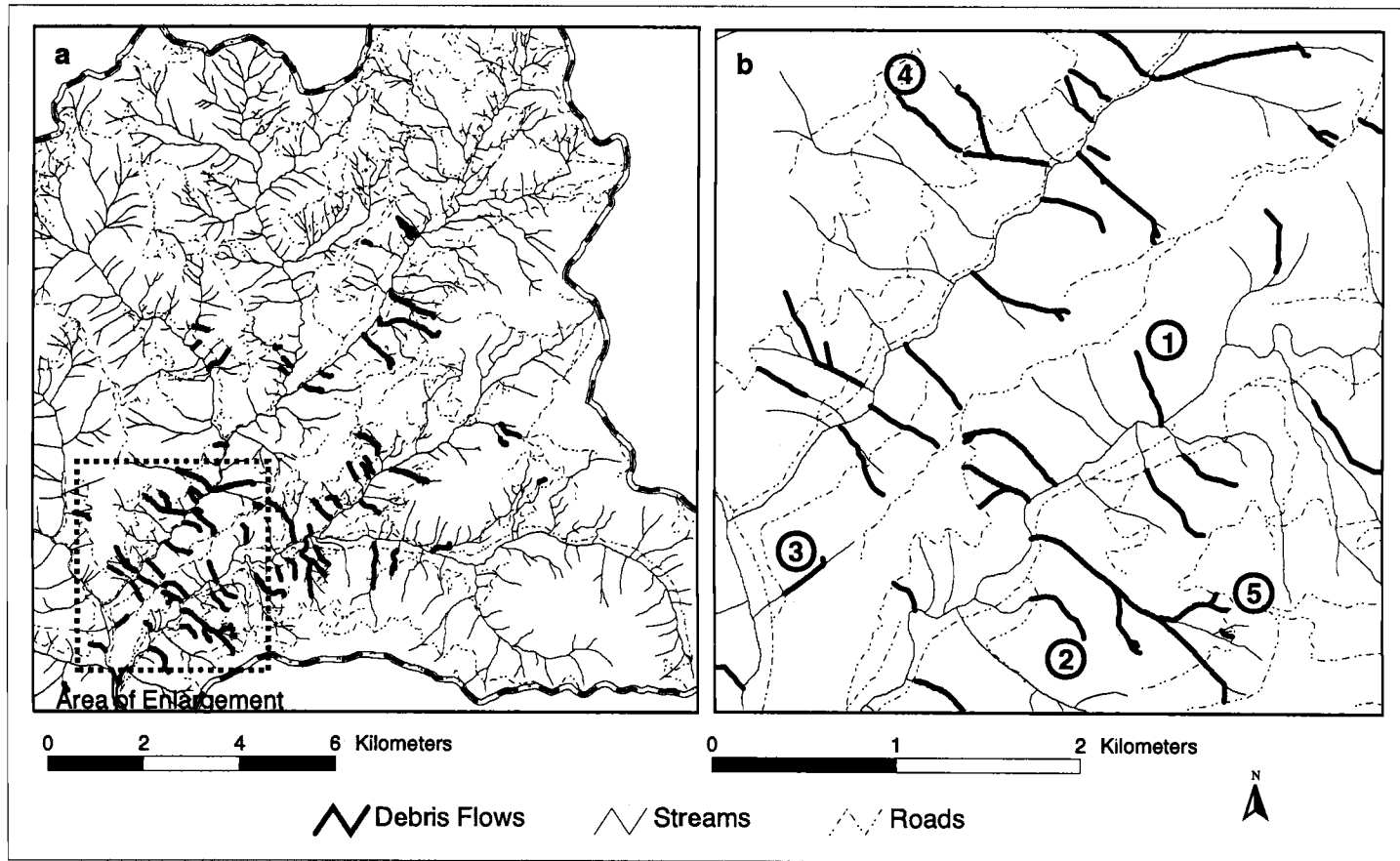
Figure 7. Patterns and types of debris flow disturbance in the stream network. See text for description of numbered types in b.
